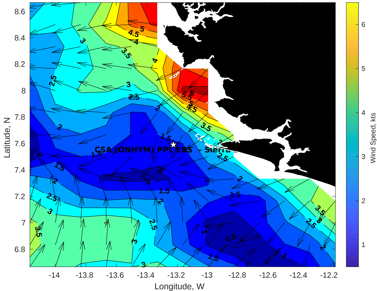
GFS Winds (kts) for CSA (ONHYM) PPL EBS - Sierra Leone at 05-Dec-2025 09:00:00
