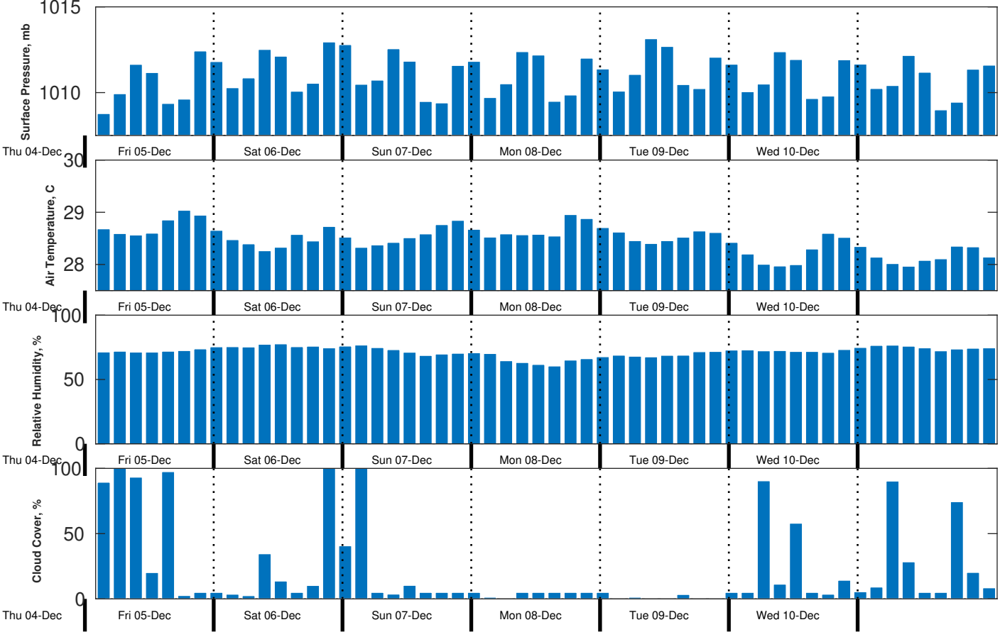
Met Forecast for CSA (ONHYM) PPL EBS - Sierra Leone from 05-Dec-2025 00:00:00 to 12-Dec-2025 00:00:00
