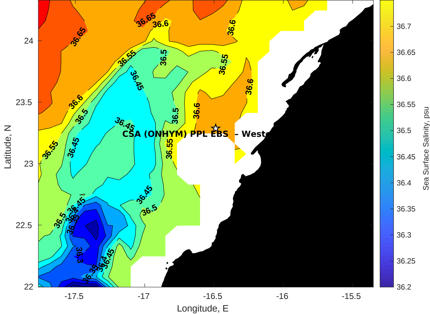
Surface Salinity for CSA (ONHYM) PPL EBS - Western Sahara at 04-Dec-2025 00:00:00
