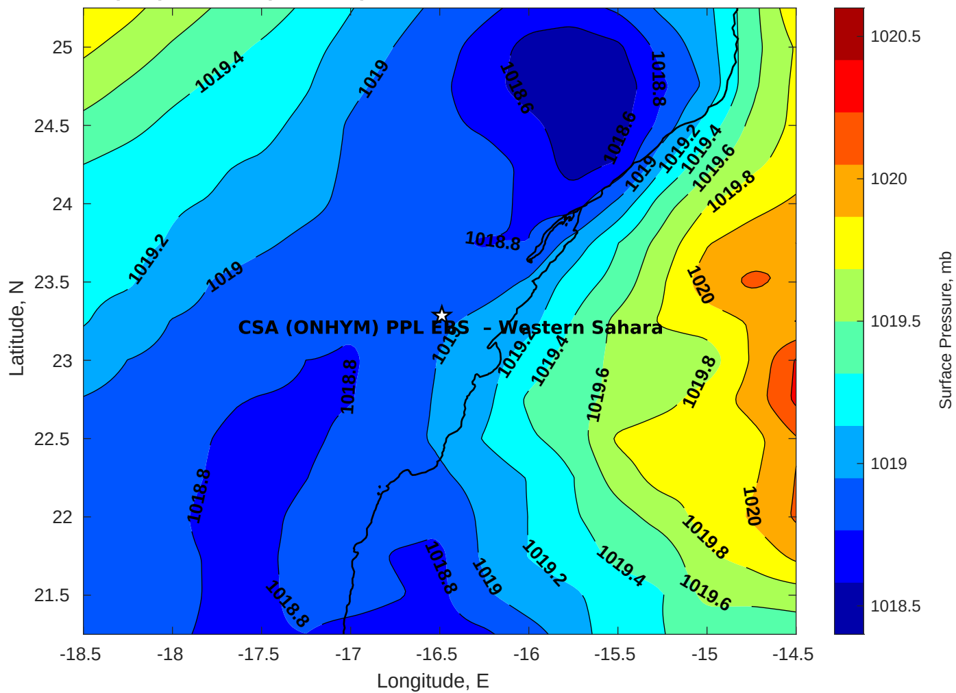
Surface Pressure (mb) for CSA (ONHYM) PPL EBS - Western Sahara at 07-Dec-2025 00:00:00
