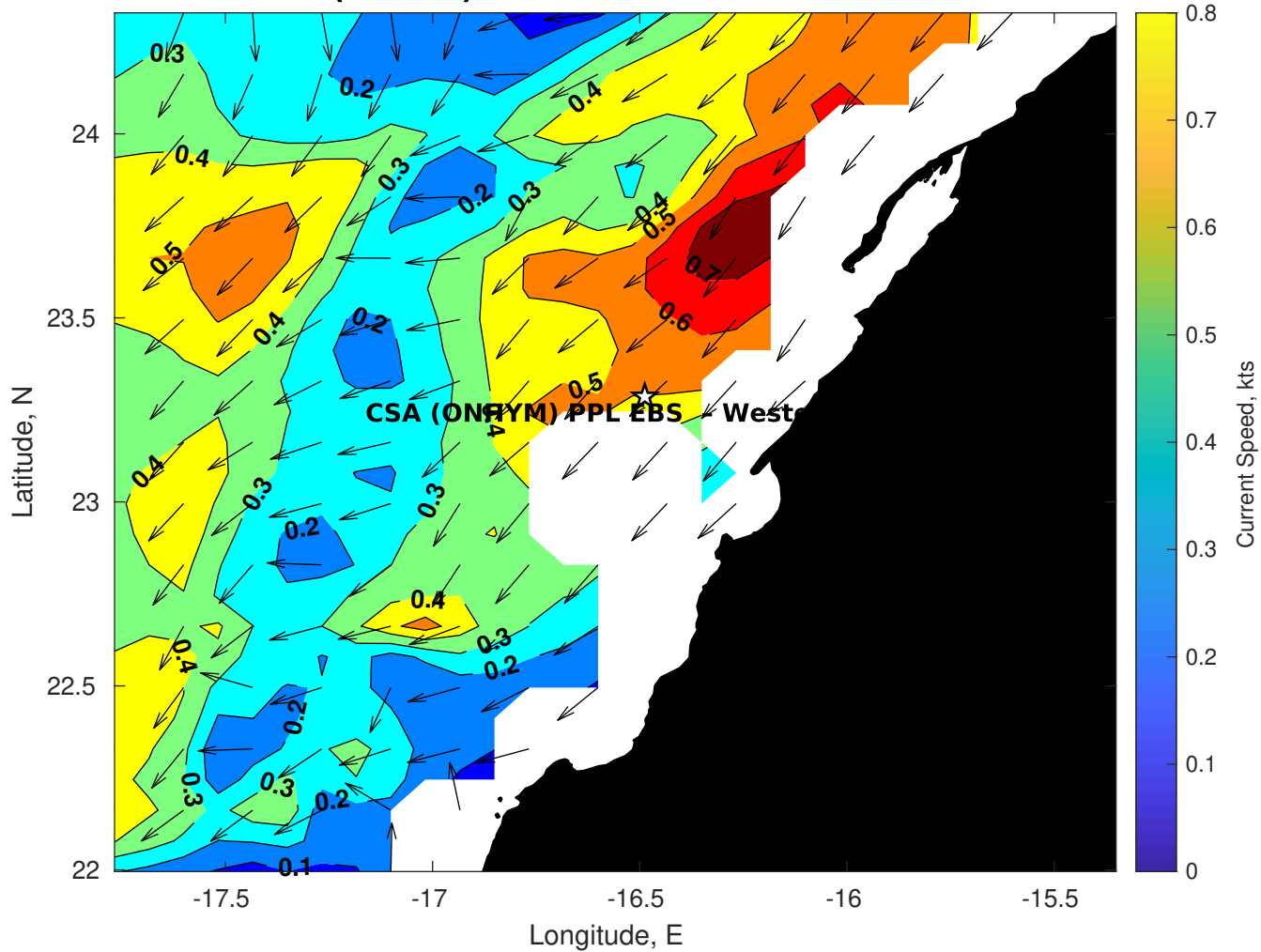
Surface Currents for CSA (ONHYM) PPL EBS - Western Sahara at 04-Dec-2025 00:00:00
