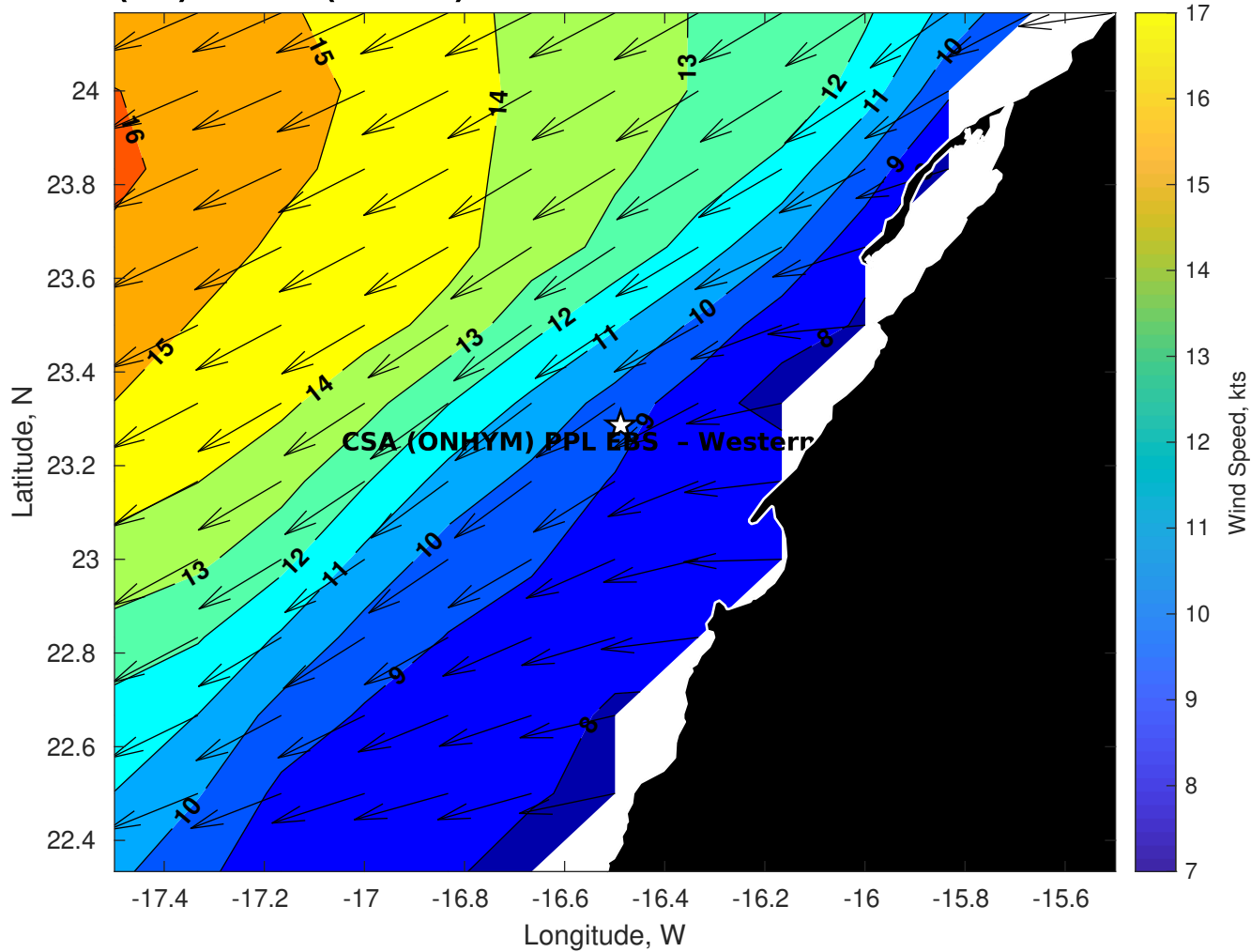
GFS Winds (kts) for CSA (ONHYM) PPL EBS - Western Sahara at 05-Dec-2025 09:00:00
