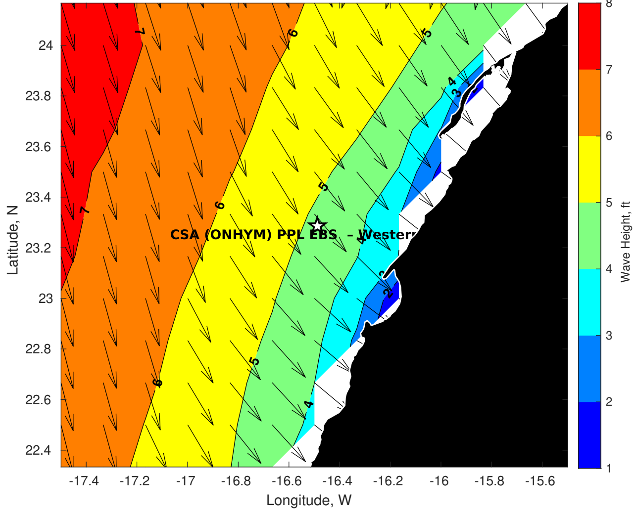
GFS Wave Height (ft) for CSA (ONHYM) PPL EBS - Western Sahara at 05-Dec-2025 09:00:00
