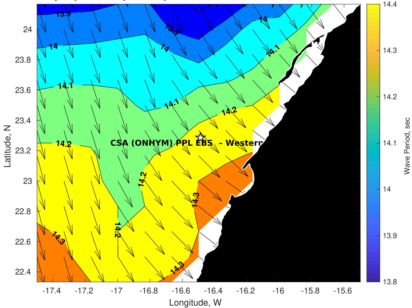
GFS Wave Period (sec) for CSA (ONHYM) PPL EBS - Western Sahara at 05-Dec-2025 09:00:00
