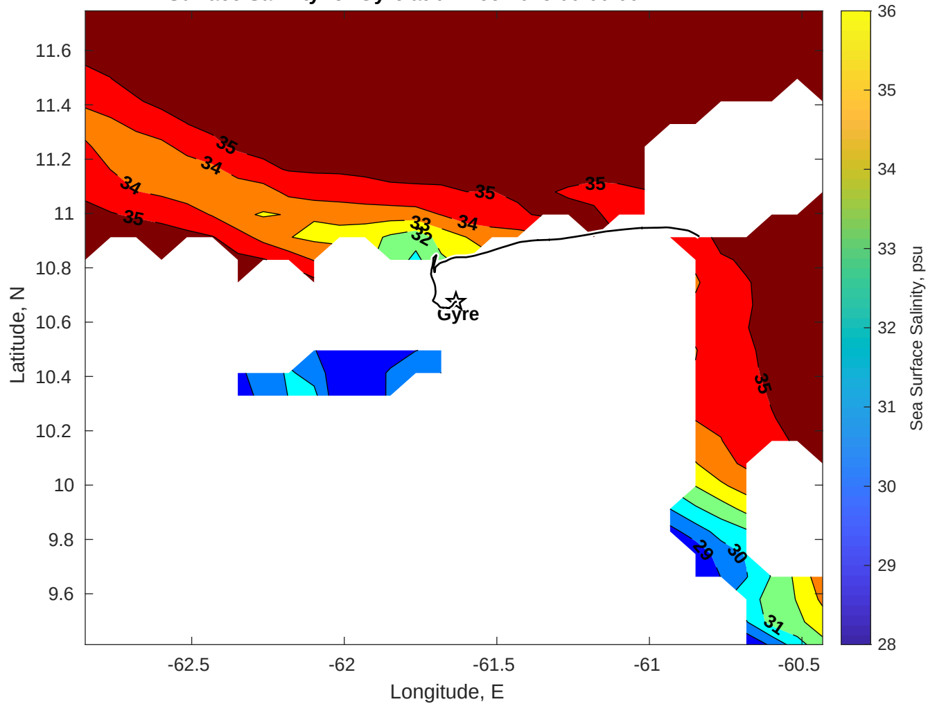
Surface Salinity for Gyre at 04-Dec-2025 00:00:00
