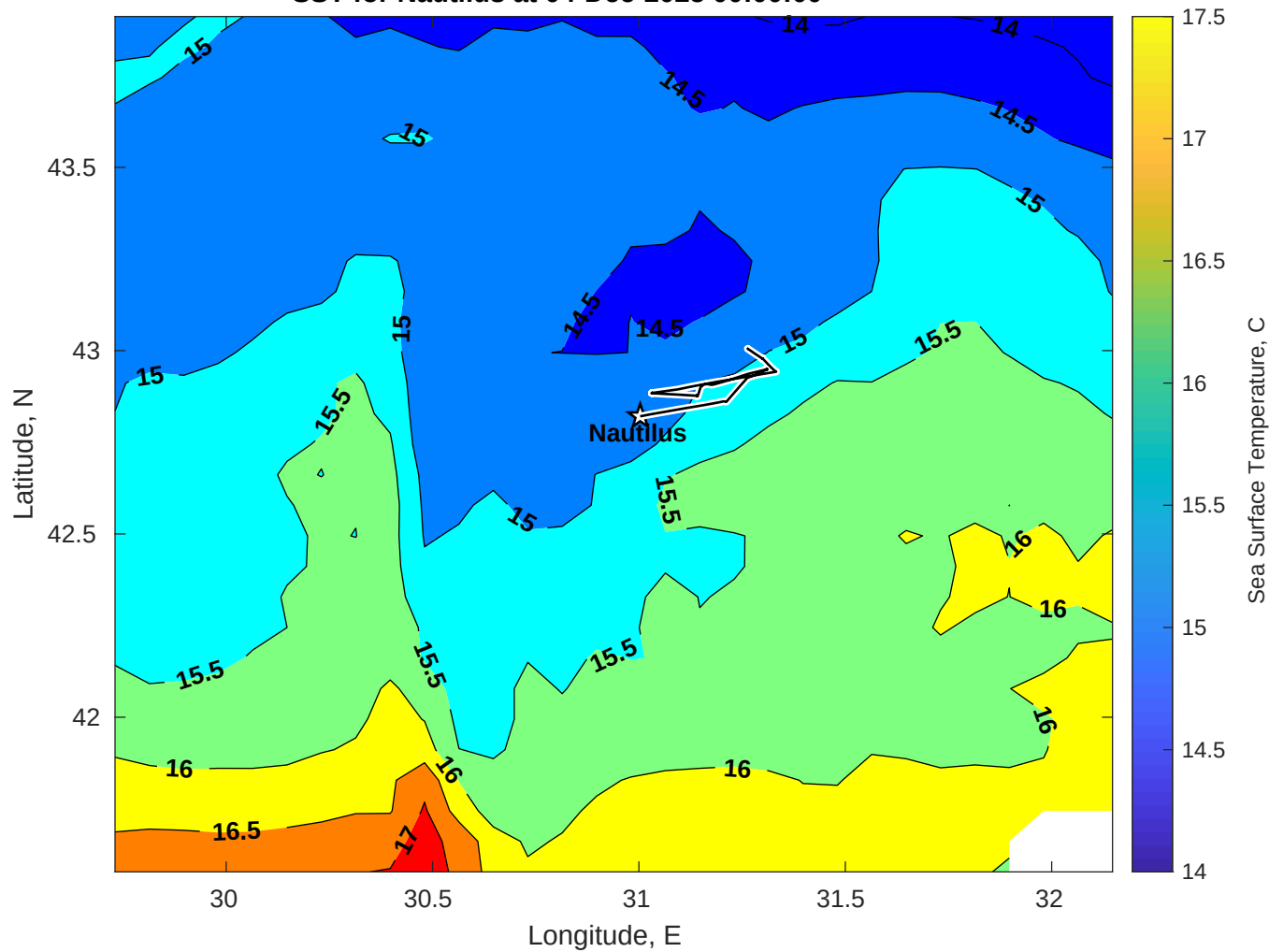
SST for Nautilus at 04-Dec-2025 00:00:00
