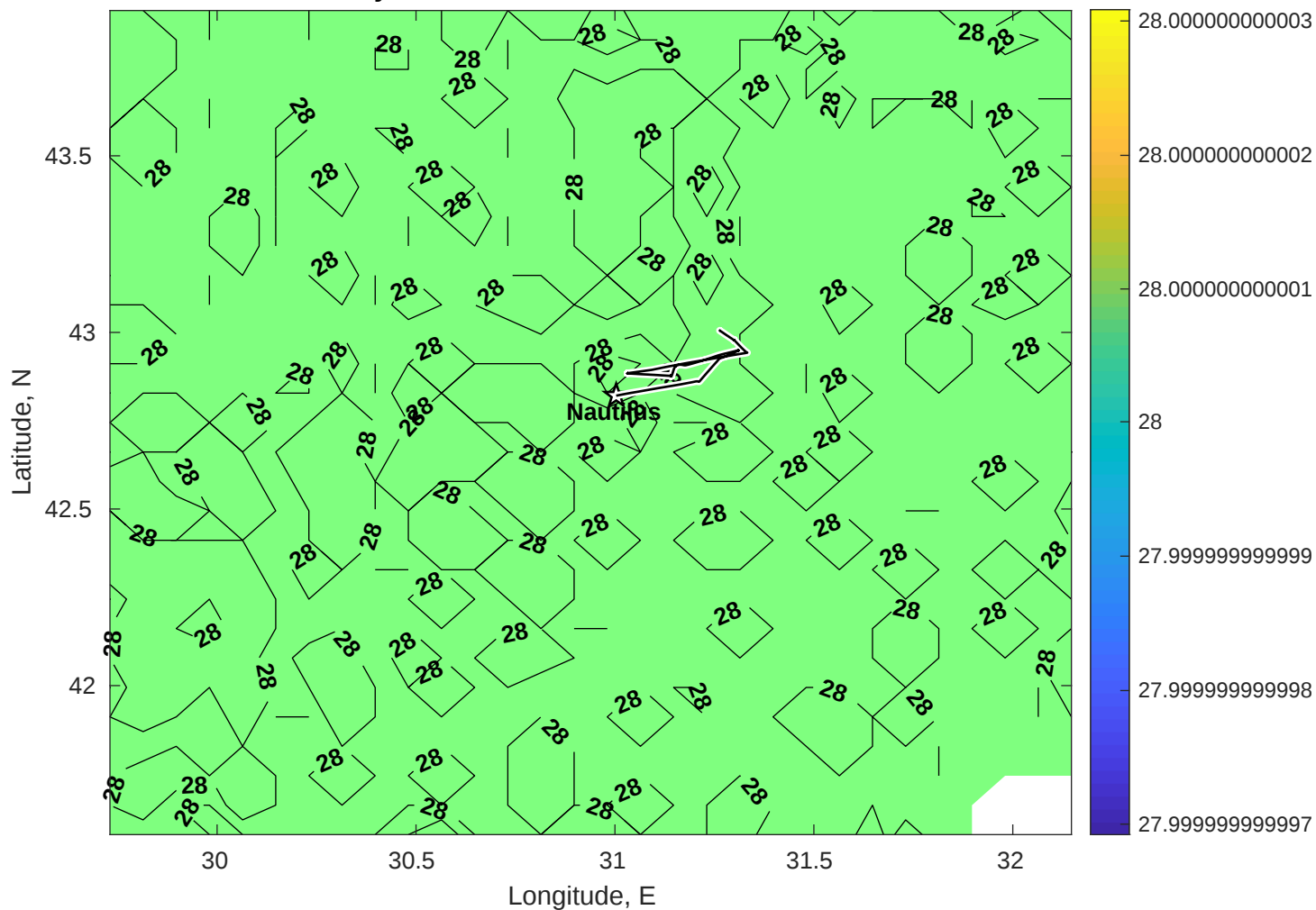
Surface Salinity for Nautilus at 04-Dec-2025 00:00:00
