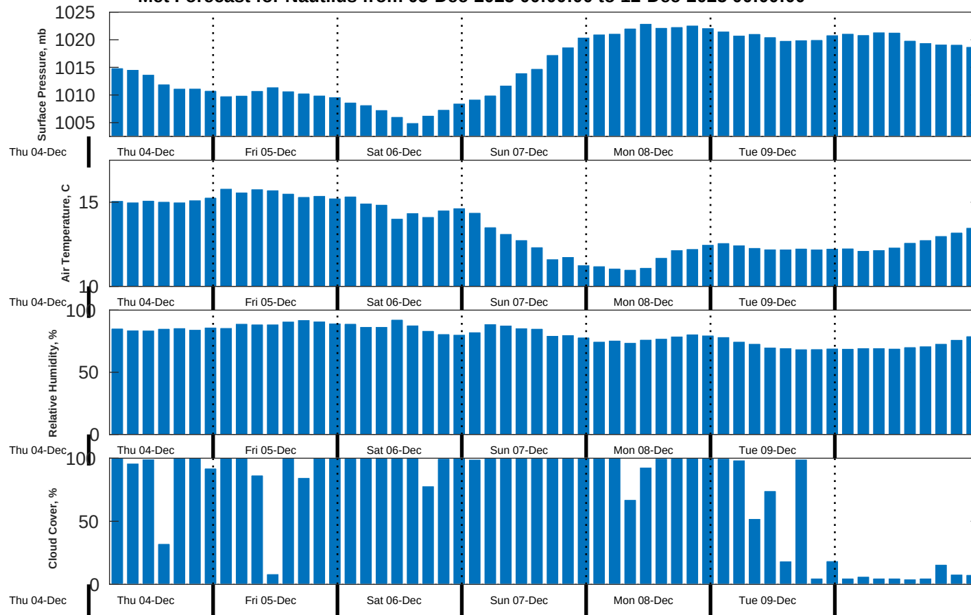
Met Forecast for Nautilus from 05-Dec-2025 00:00:00 to 12-Dec-2025 00:00:00
