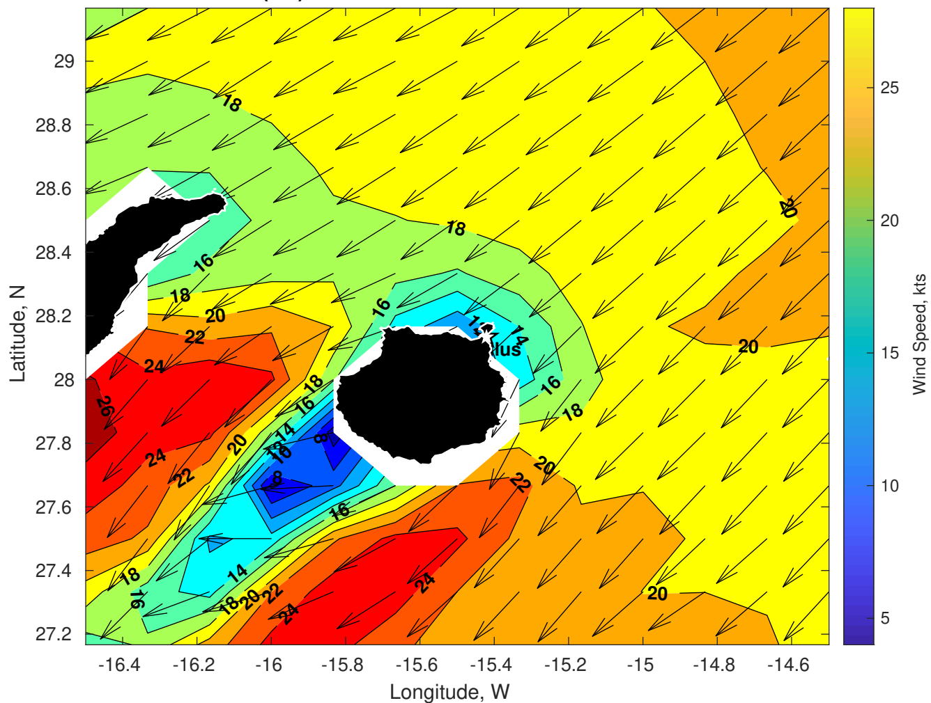
GFS Winds (kts) for Nautilus at 03-Dec-2025 21:00:00
