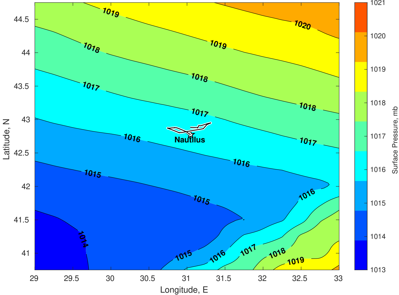
Surface Pressure (mb) for Nautilus at 05-Dec-2025 00:00:00
