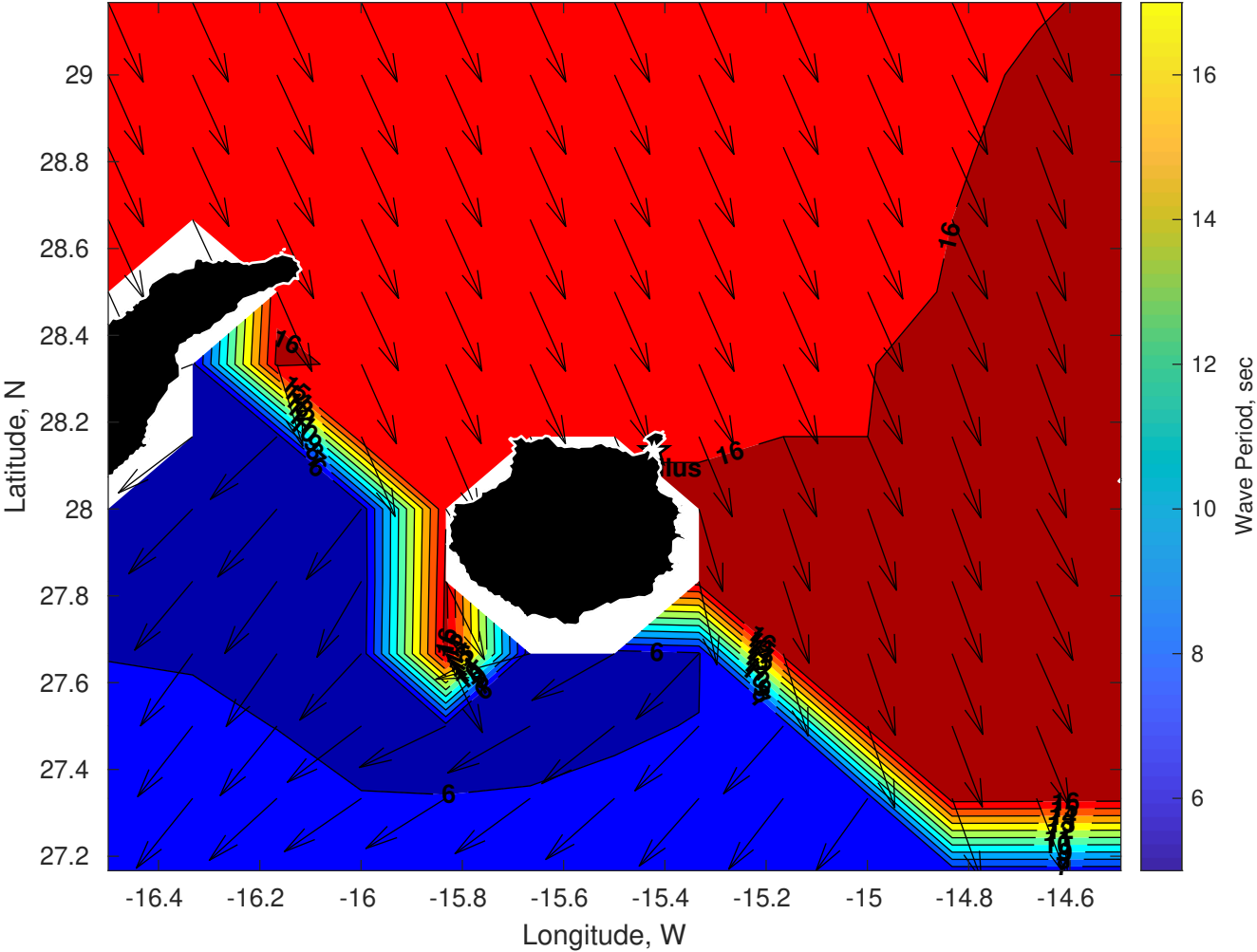
GFS Wave Period (sec) for Nautilus at 03-Dec-2025 21:00:00
