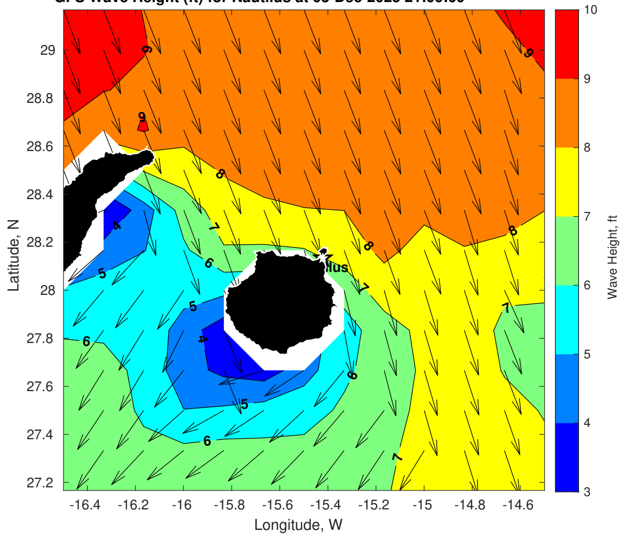
GFS Wave Height (ft) for Nautilus at 03-Dec-2025 21:00:00
