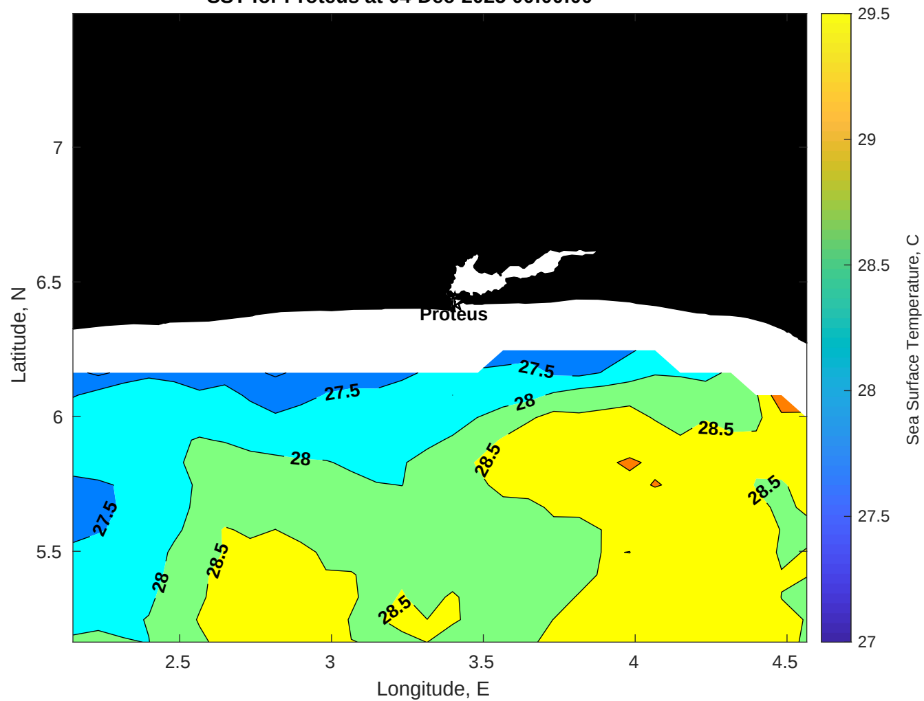
SST for Proteus at 04-Dec-2025 00:00:00
