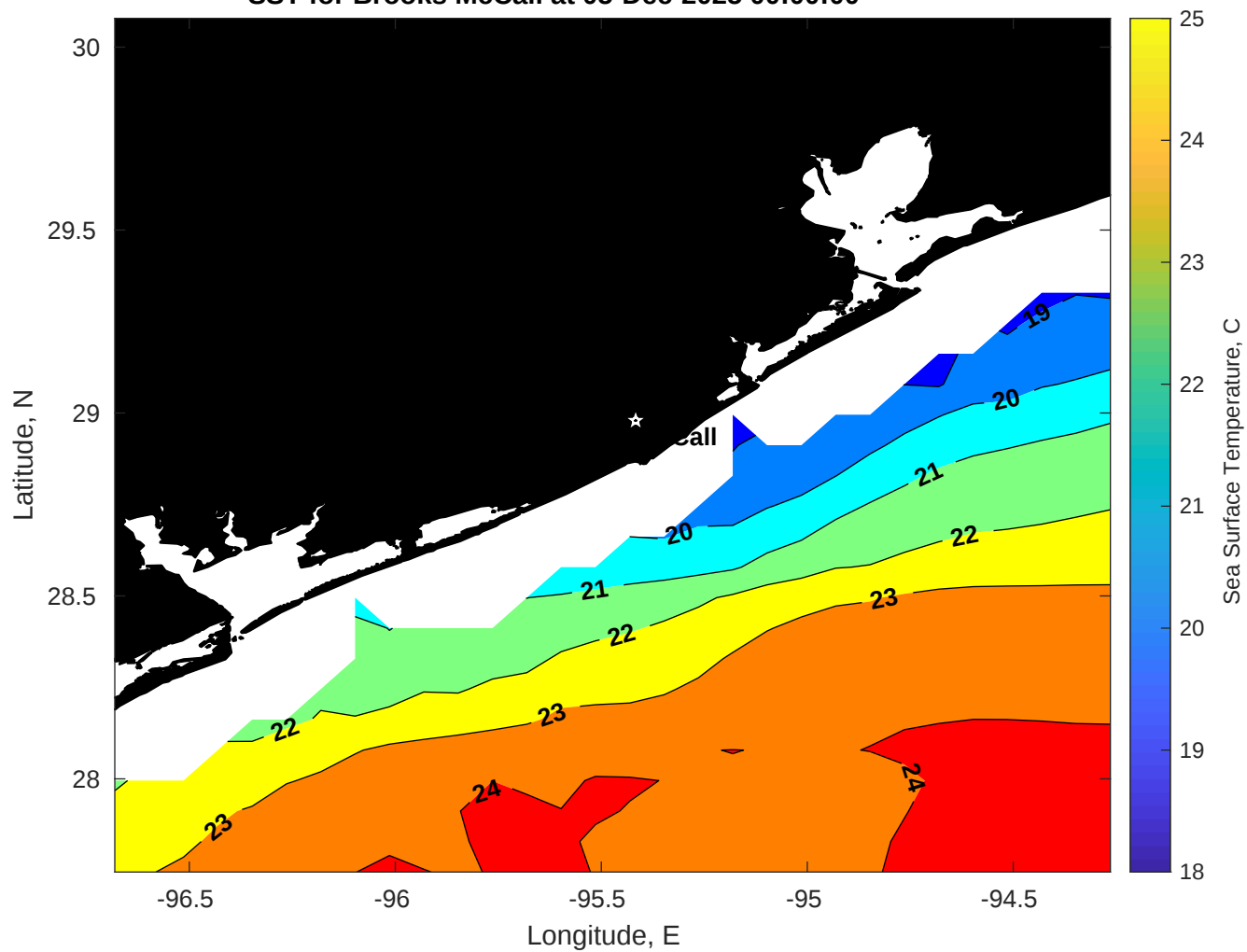
SST for Brooks McCall at 05-Dec-2025 00:00:00
