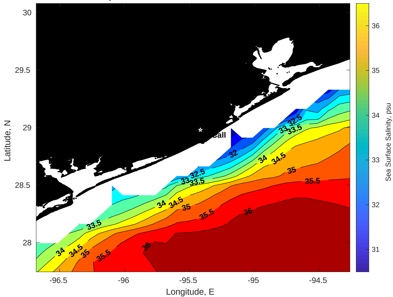
Surface Salinity for Brooks McCall at 05-Dec-2025 00:00:00
