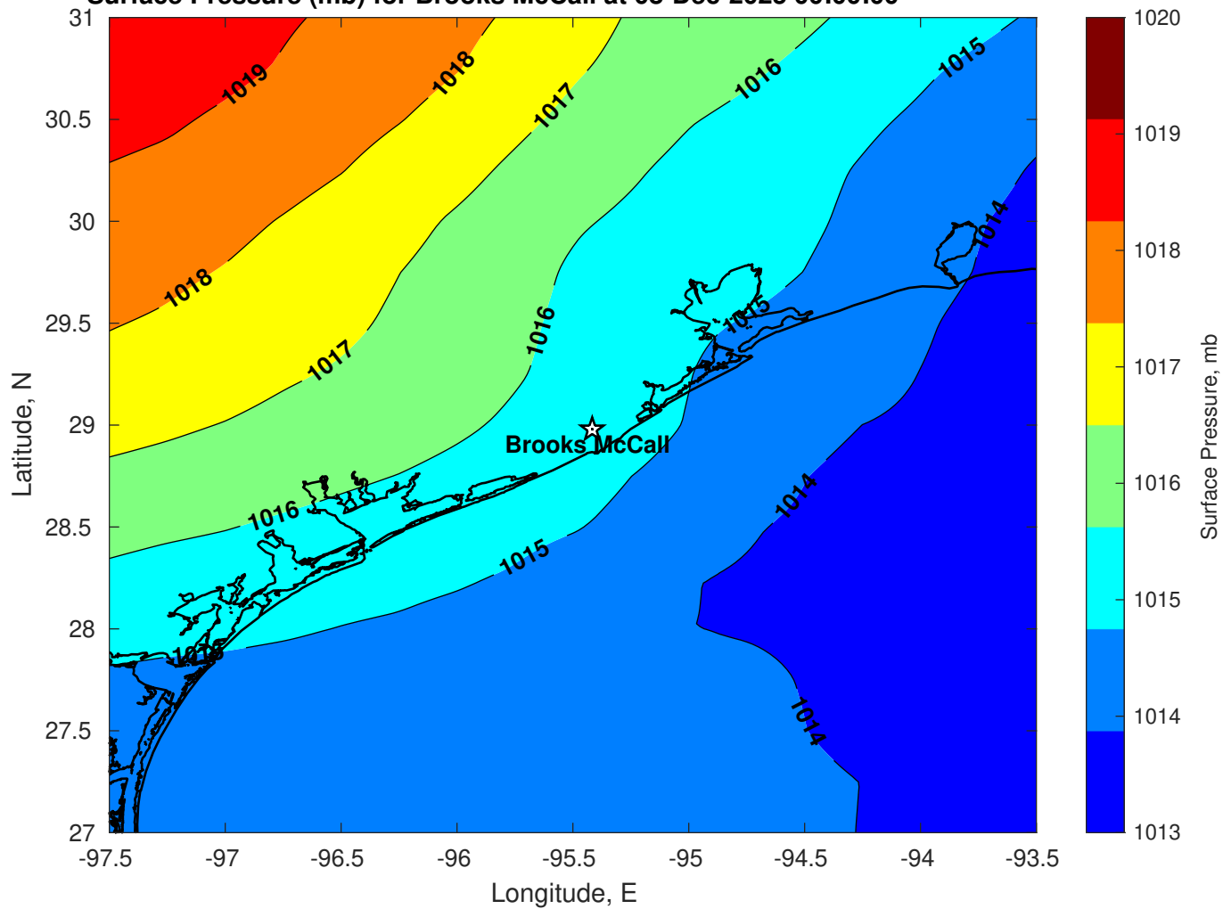
Surface Pressure (mb) for Brooks McCall at 08-Dec-2025 00:00:00
