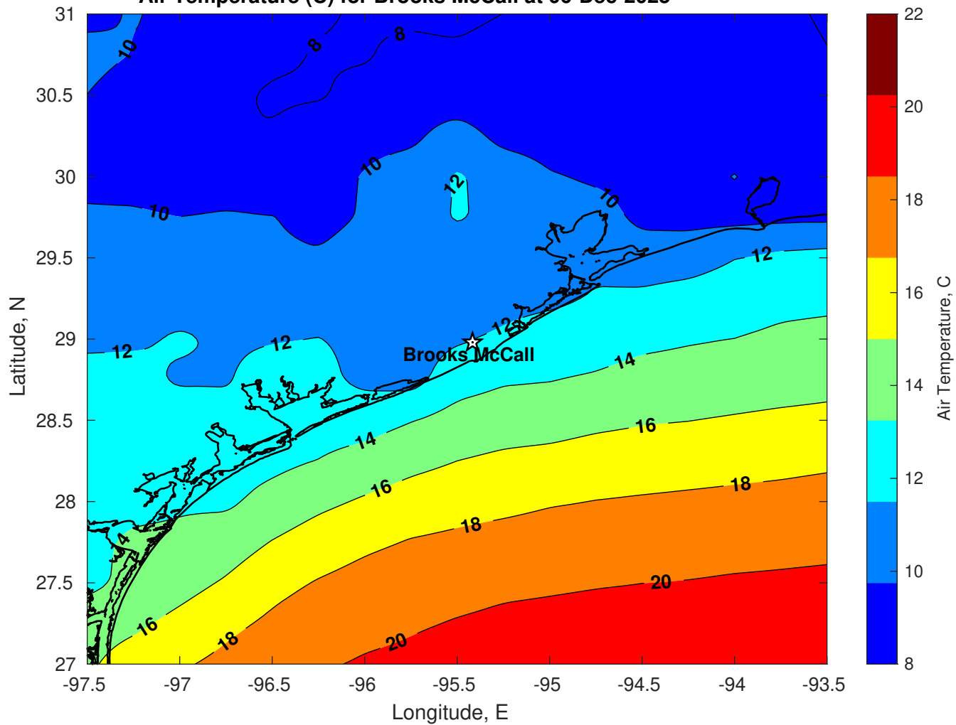
Air Temperature (C) for Brooks McCall at 06-Dec-2025
