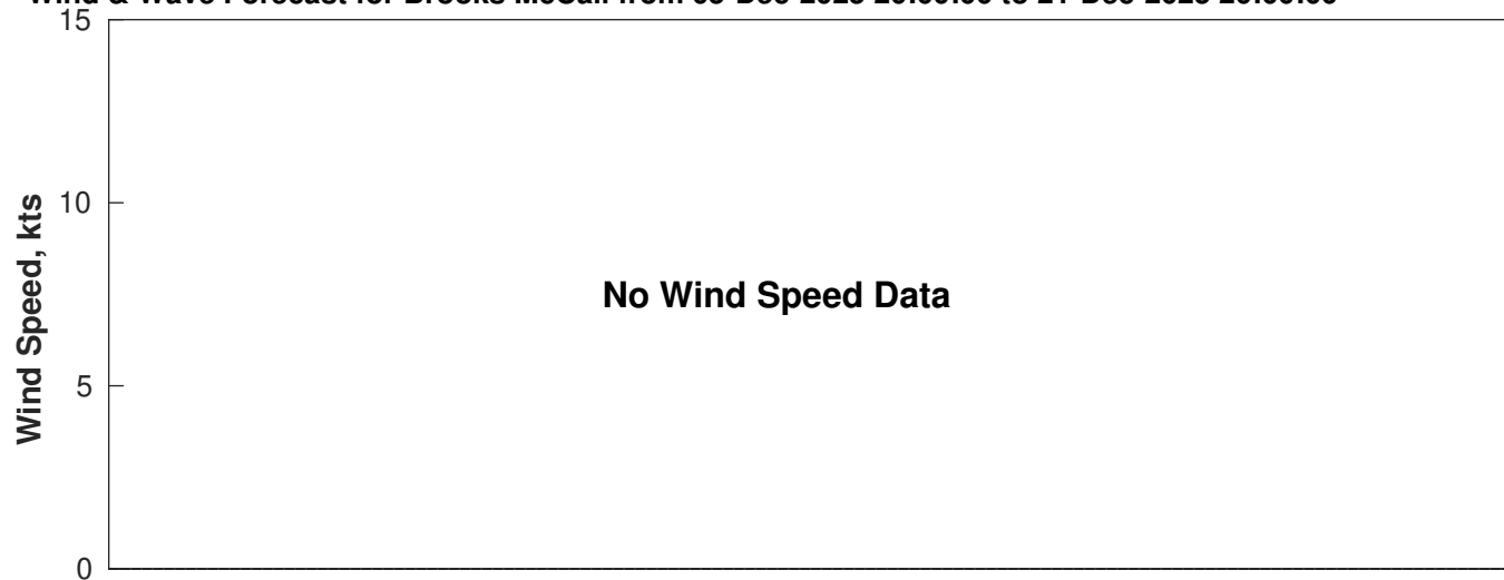
Wind & Wave Forecast for Brooks McCall from 05-Dec-2025 20:00:00 to 21-Dec-2025 20:00:00
