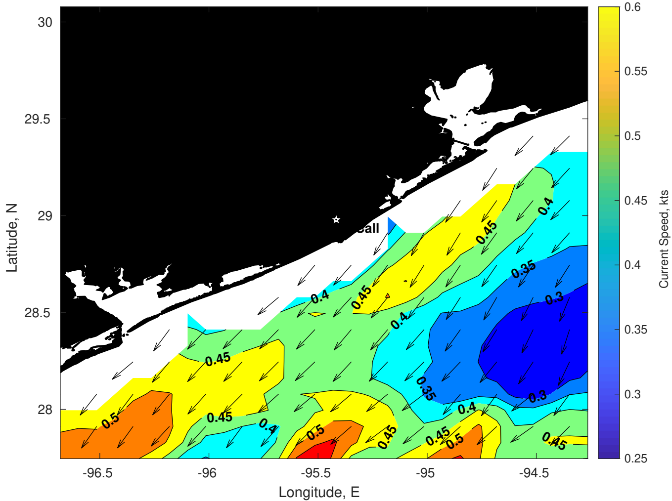
Surface Currents for Brooks McCall at 05-Dec-2025 00:00:00
