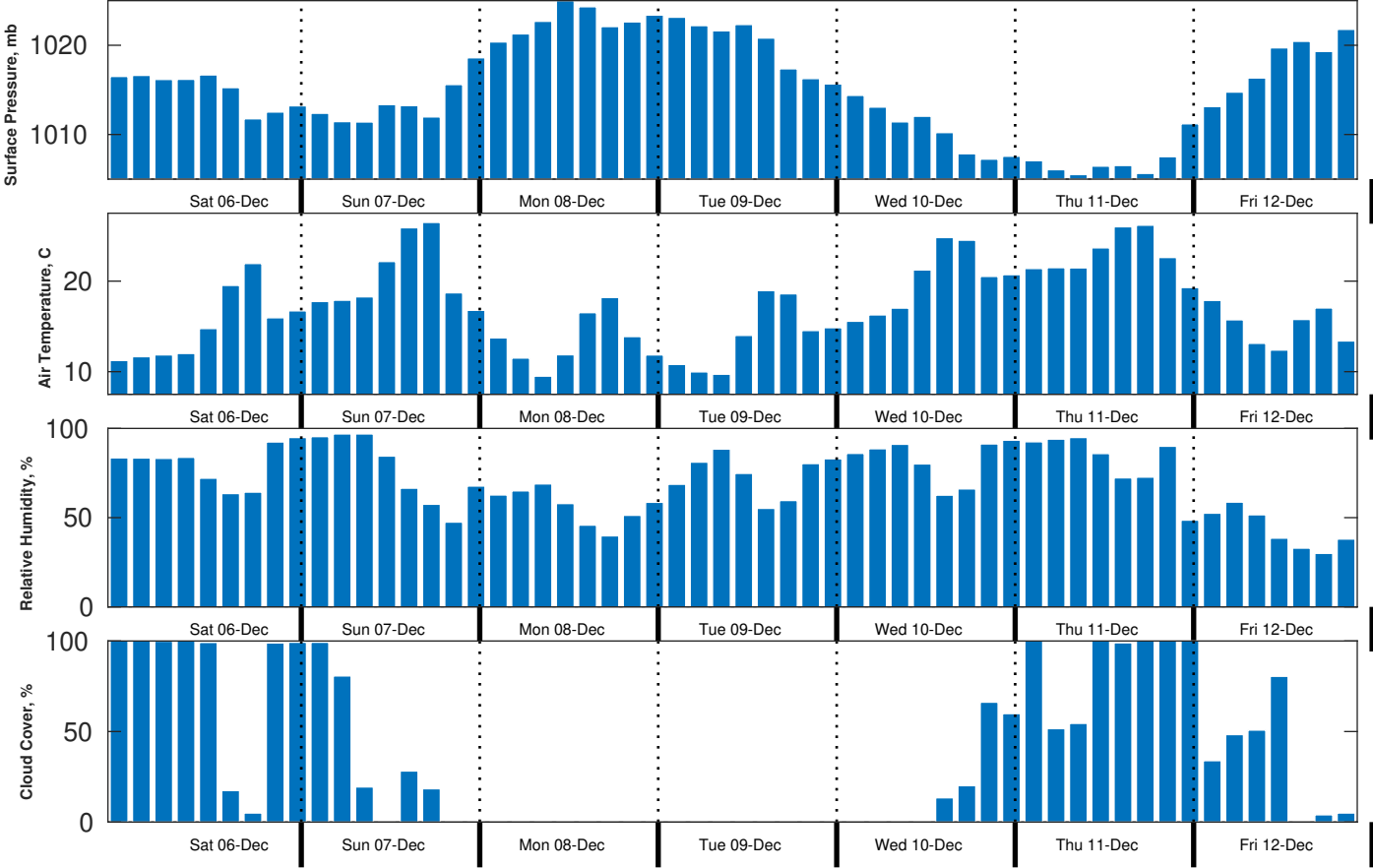
Met Forecast for Brooks McCall from 06-Dec-2025 00:00:00 to 13-Dec-2025 00:00:00
