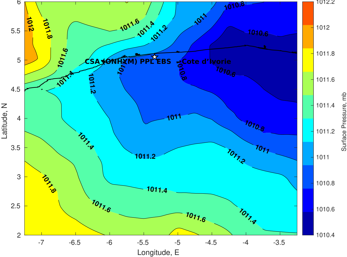
Surface Pressure (mb) for CSA (ONHYM) PPL EBS - Cote d'Ivoire at 08-Dec-2025 00:00:00
