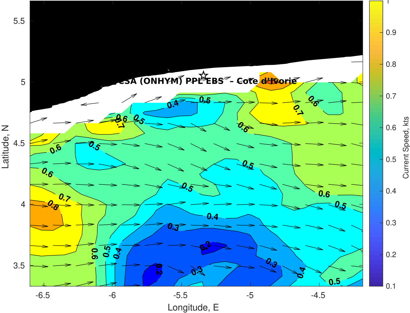
Surface Currents for CSA (ONHYM) PPL EBS - Cote d'Ivoire at 05-Dec-2025 00:00:00
