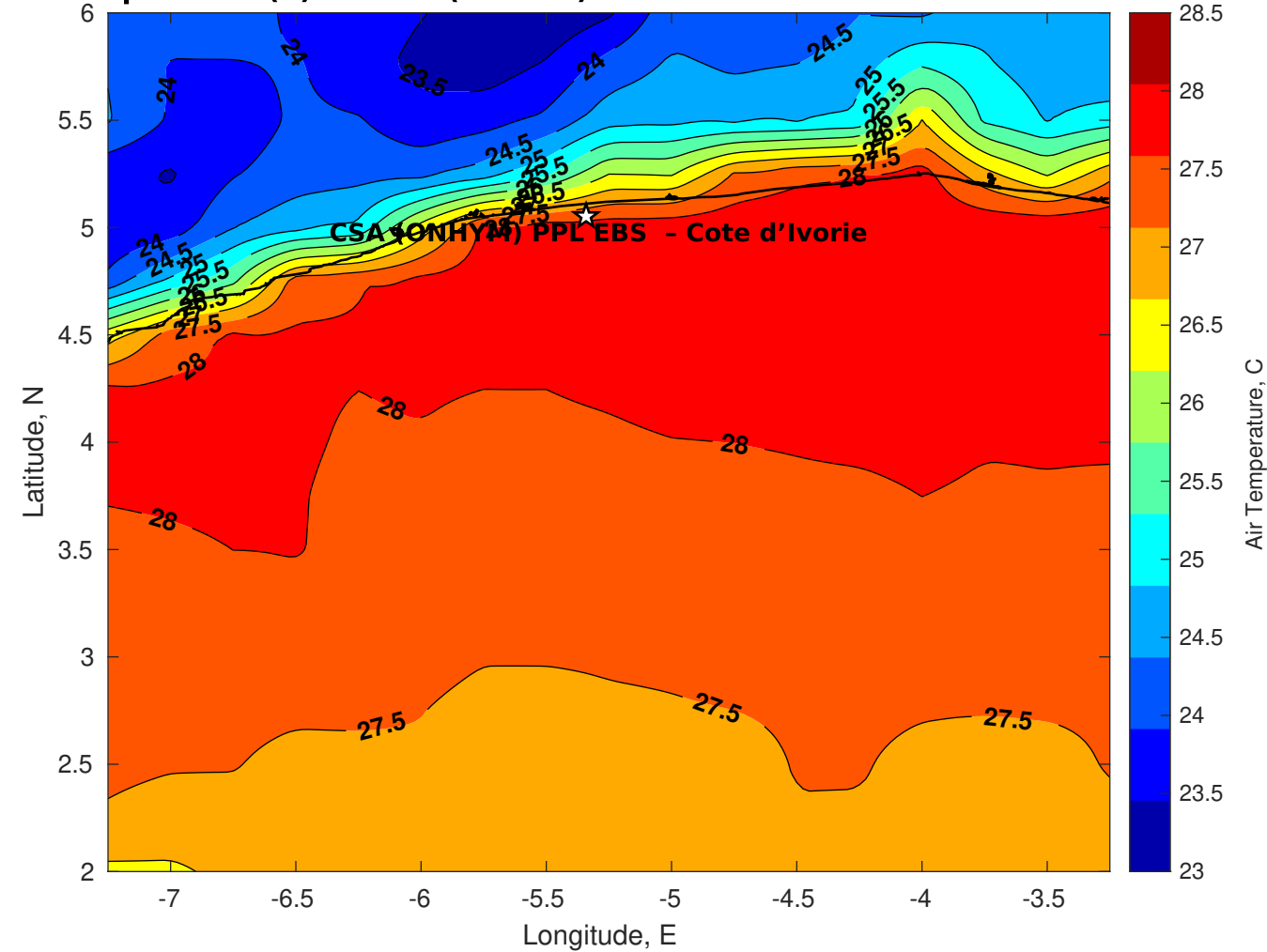
Air Temperature (C) for CSA (ONHYM) PPL EBS - Cote d'Ivoire at 06-Dec-2025
