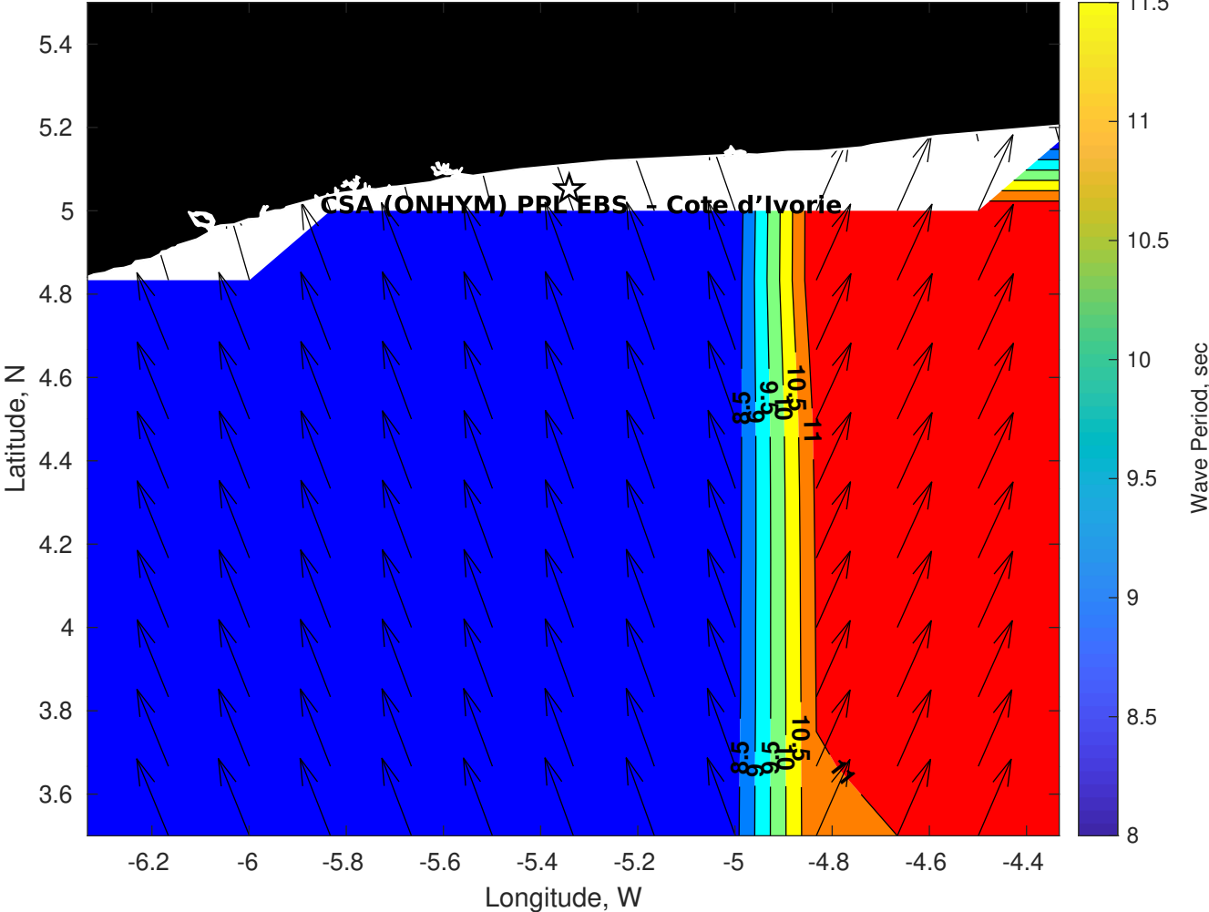
GFS Wave Period (sec) for CSA (ONHYM) PPL EBS - Cote d'Ivoire at 06-Dec-2025 09:00:00
