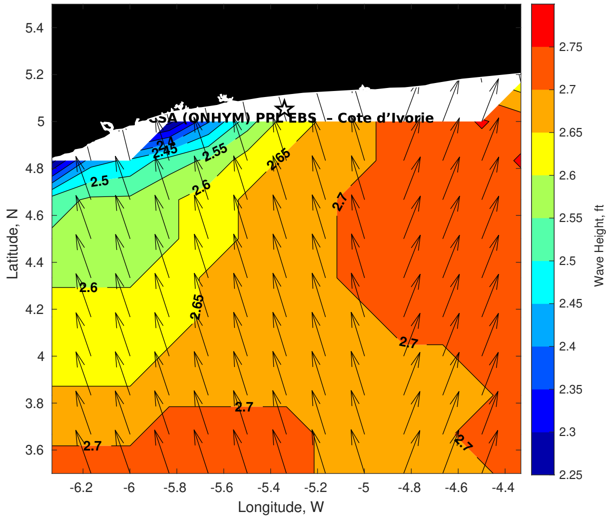
GFS Wave Height (ft) for CSA (ONHYM) PPL EBS - Cote d'Ivoire at 06-Dec-2025 09:00:00
