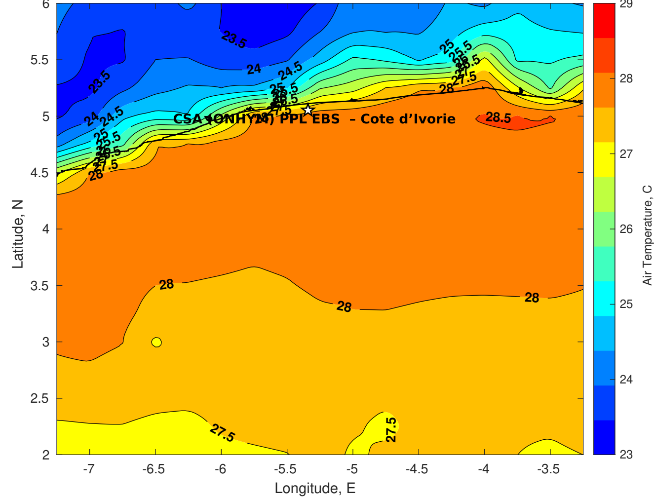
Air Temperature (C) for CSA (ONHYM) PPL EBS - Cote d'Ivoire at 06-Dec-2025
