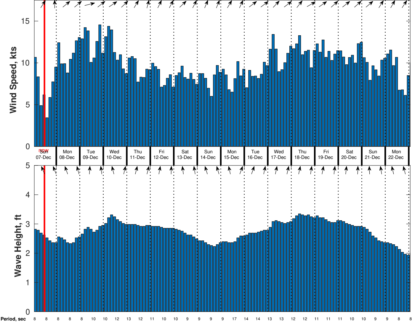
Wind & Wave Forecast for CSA (ONHYM) PPL EBS - Cote d'Ivoire from 06-Dec-2025 01:00:00 to 22-Dec-2025 01:00:00
