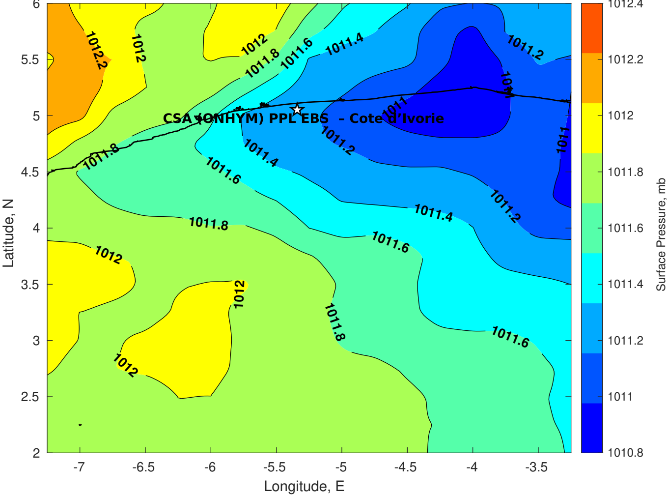
Surface Pressure (mb) for CSA (ONHYM) PPL EBS - Cote d'Ivoire at 07-Dec-2025 00:00:00
