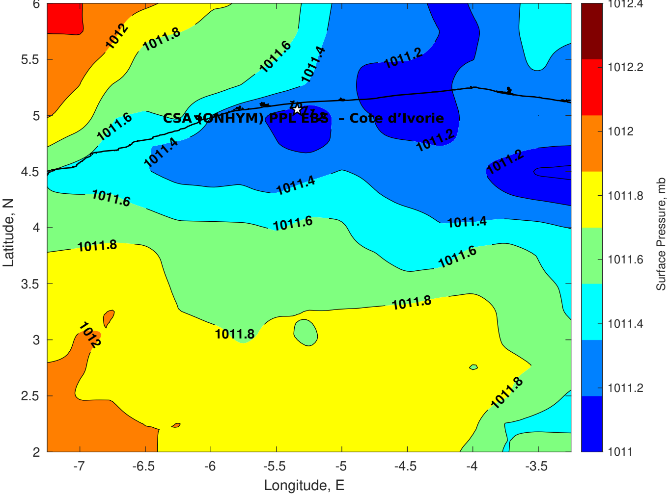
Surface Pressure (mb) for CSA (ONHYM) PPL EBS - Cote d'Ivoire at 06-Dec-2025 00:00:00
