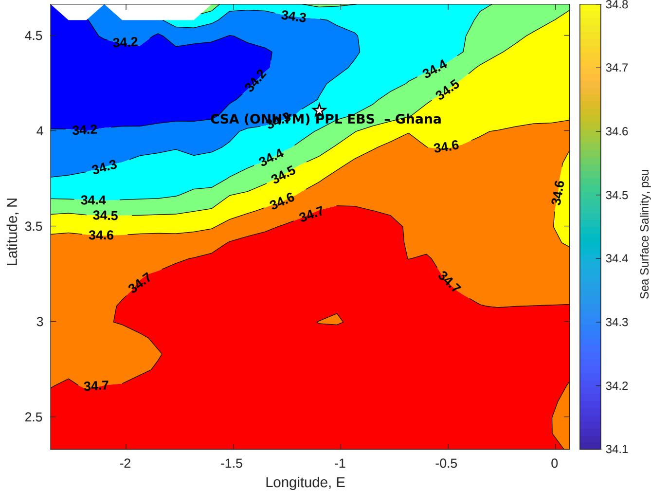
Surface Salinity for CSA (ONHYM) PPL EBS - Ghana at 05-Dec-2025 00:00:00
