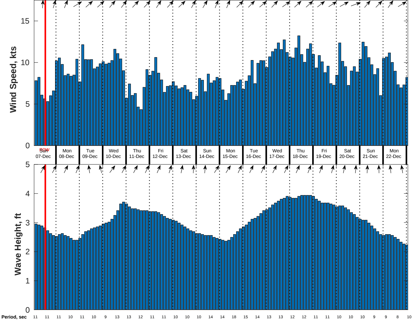
Wind & Wave Forecast for CSA (ONHYM) PPL EBS - Ghana from 06-Dec-2025 02:00:00 to 22-Dec-2025 02:00:00
