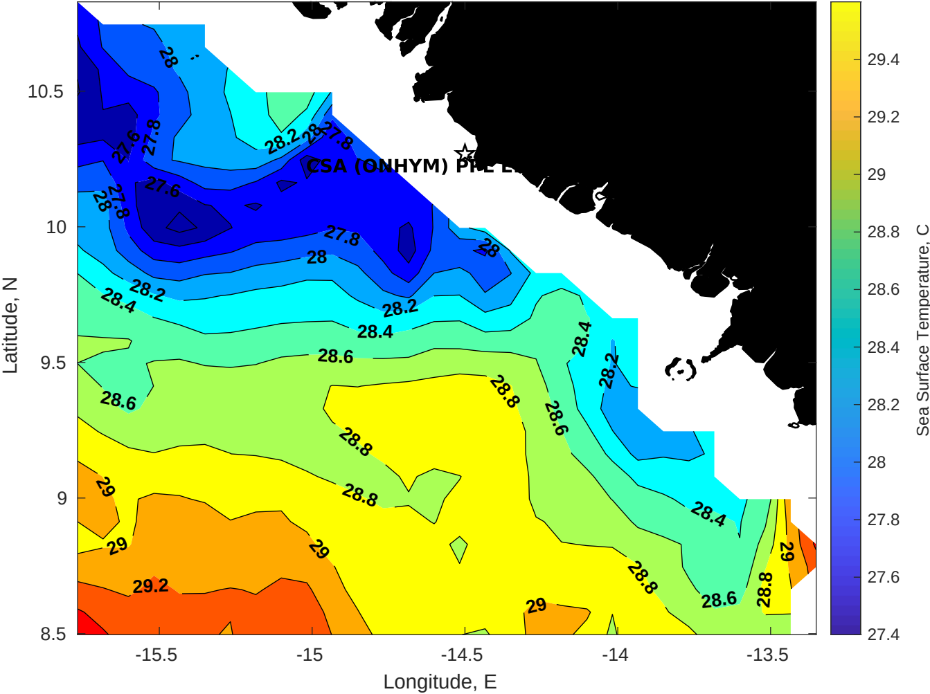
SST for CSA (ONHYM) PPL EBS - Guinea at 05-Dec-2025 00:00:00
