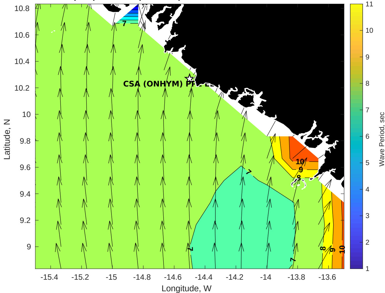
GFS Wave Period (sec) for CSA (ONHYM) PPL EBS - Guinea at 06-Dec-2025 09:00:00
