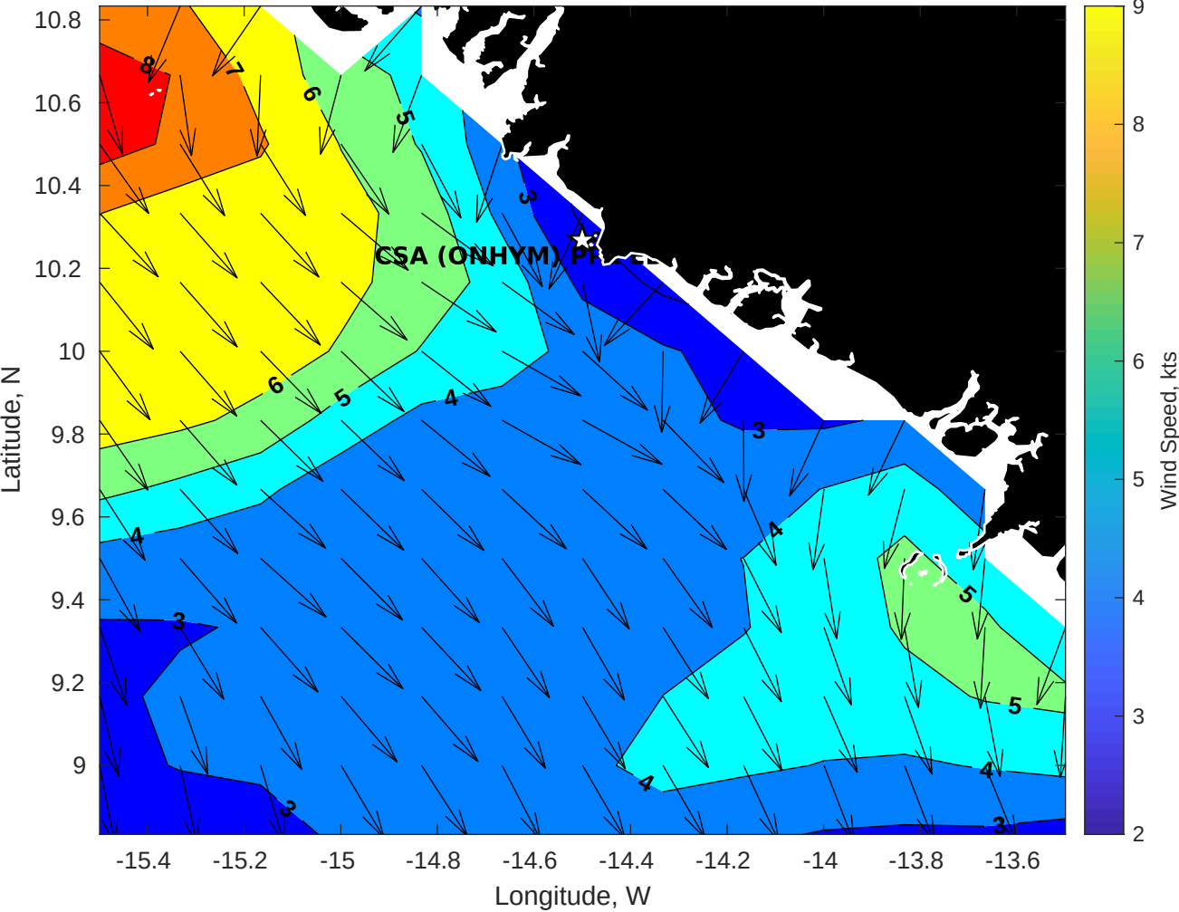
GFS Winds (kts) for CSA (ONHYM) PPL EBS - Guinea at 06-Dec-2025 09:00:00
