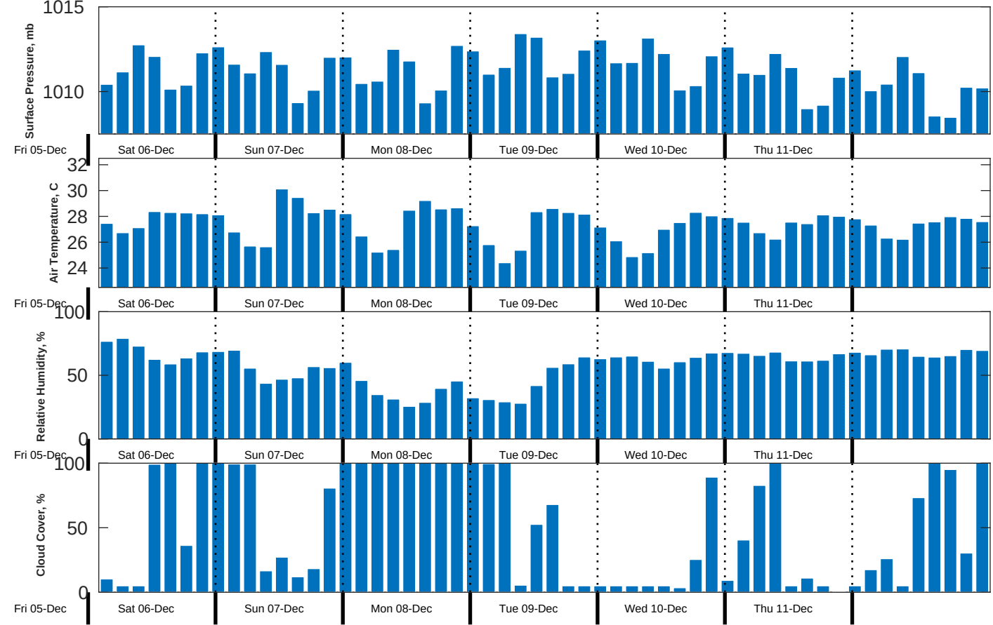
Met Forecast for CSA (ONHYM) PPL EBS - Guinea from 06-Dec-2025 00:00:00 to 13-Dec-2025 00:00:00
