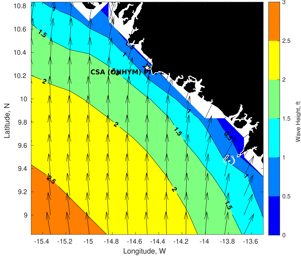
GFS Wave Height (ft) for CSA (ONHYM) PPL EBS - Guinea at 06-Dec-2025 09:00:00
