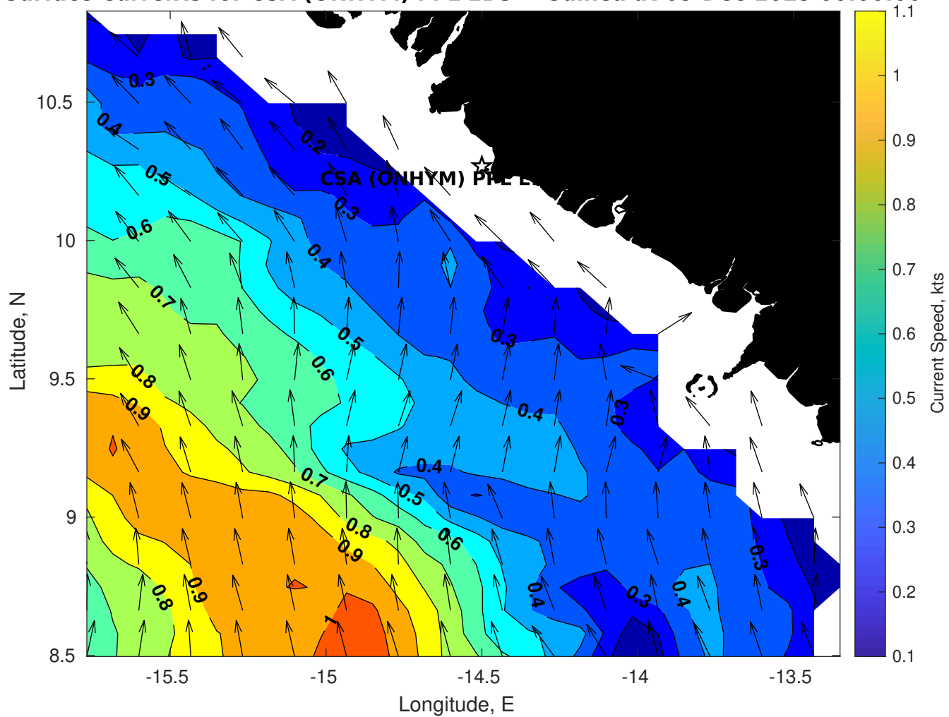
Surface Currents for CSA (ONHYM) PPL EBS - Guinea at 05-Dec-2025 00:00:00
