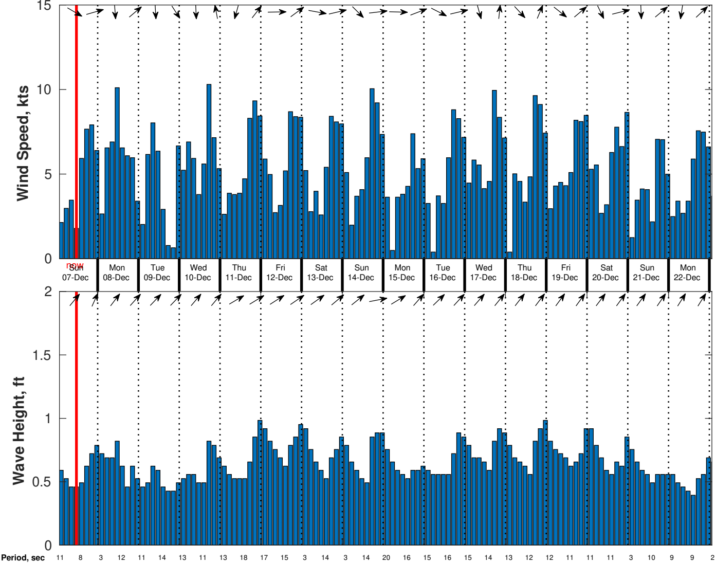
Wind & Wave Forecast for CSA (ONHYM) PPL EBS - Guinea from 06-Dec-2025 01:00:00 to 22-Dec-2025 01:00:00
