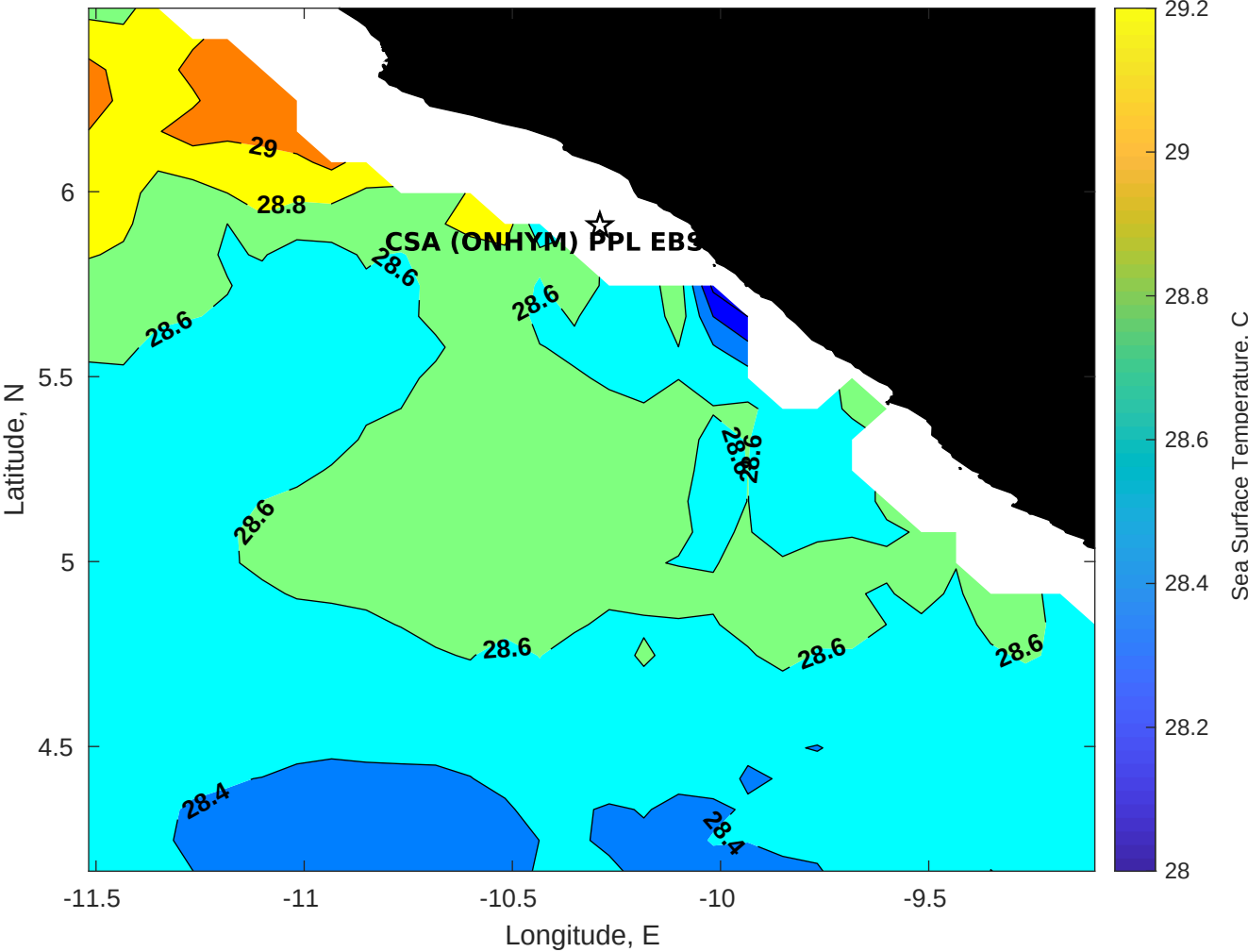
SST for CSA (ONHYM) PPL EBS - Liberia at 05-Dec-2025 00:00:00
