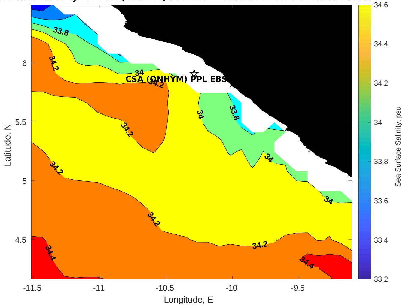
Surface Salinity for CSA (ONHYM) PPL EBS - Liberia at 05-Dec-2025 00:00:00
