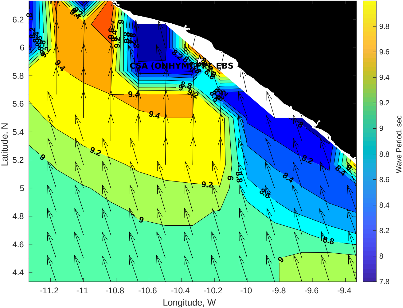
GFS Wave Period (sec) for CSA (ONHYM) PPL EBS - Liberia at 06-Dec-2025 09:00:00
