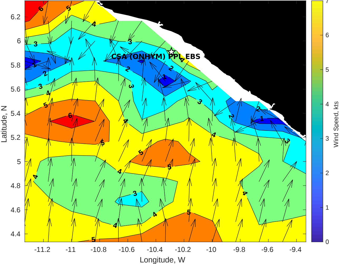
GFS Winds (kts) for CSA (ONHYM) PPL EBS - Liberia at 06-Dec-2025 09:00:00
