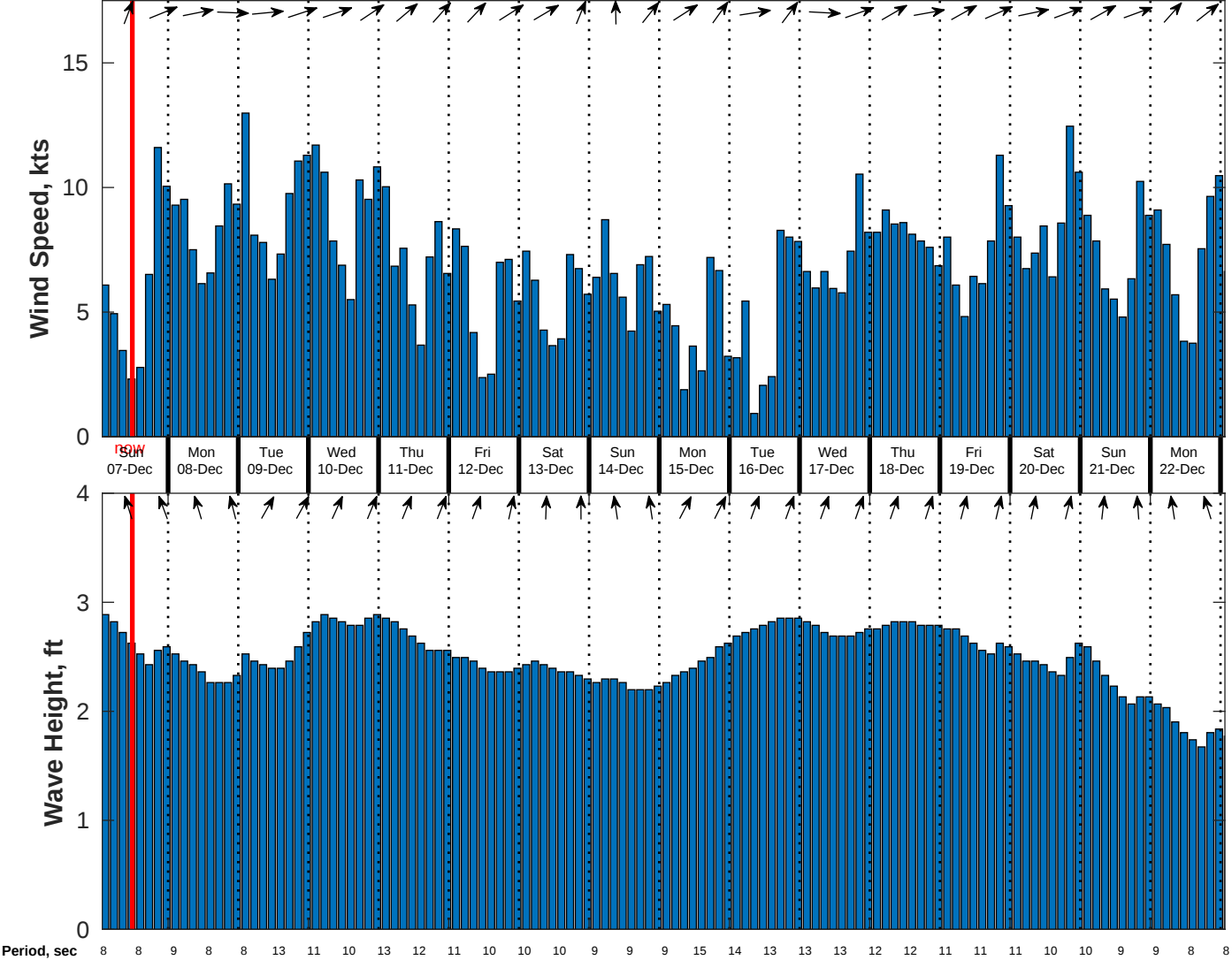
Wind & Wave Forecast for CSA (ONHYM) PPL EBS - Liberia from 06-Dec-2025 01:00:00 to 22-Dec-2025 01:00:00
