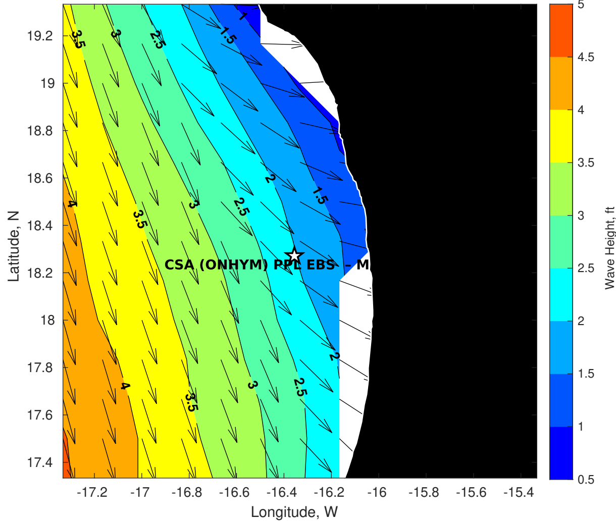
GFS Wave Height (ft) for CSA (ONHYM) PPL EBS - Mauritania at 06-Dec-2025 09:00:00
