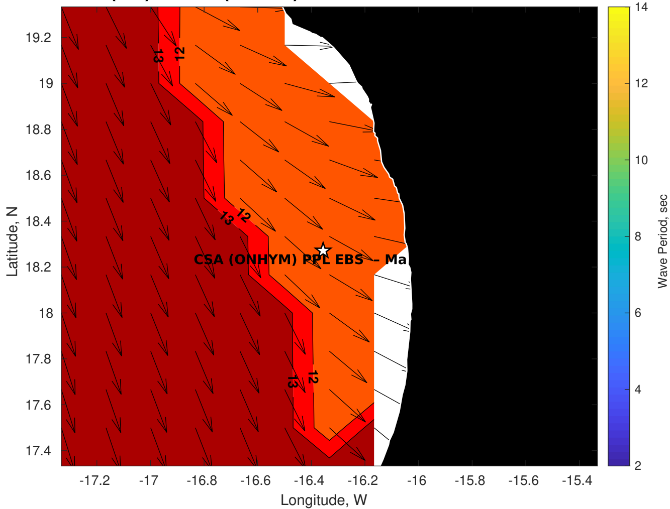
GFS Wave Period (sec) for CSA (ONHYM) PPL EBS - Mauritania at 06-Dec-2025 09:00:00
