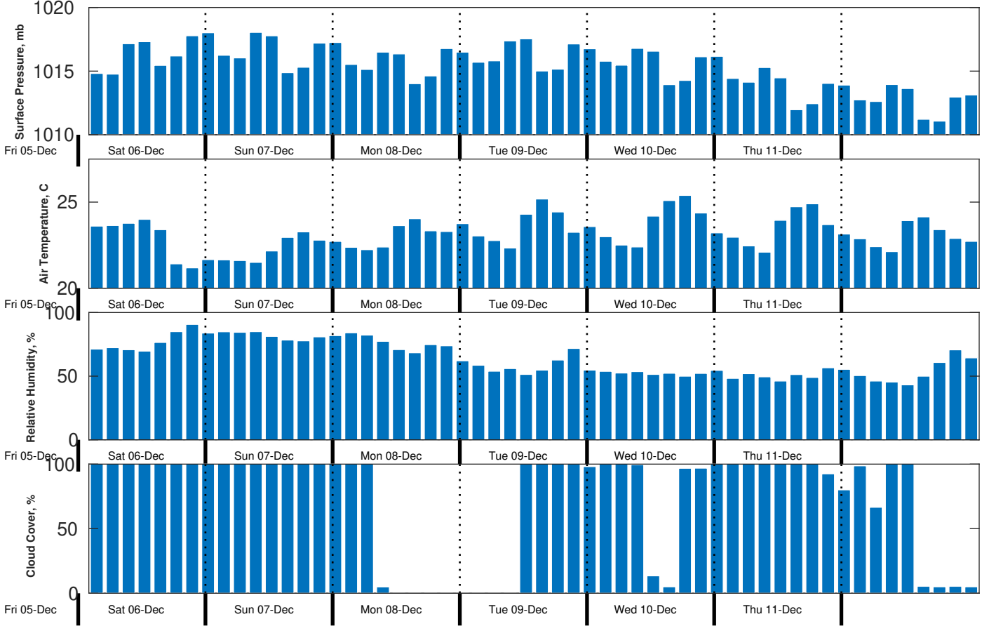
Met Forecast for CSA (ONHYM) PPL EBS - Mauritania from 06-Dec-2025 00:00:00 to 13-Dec-2025 00:00:00
