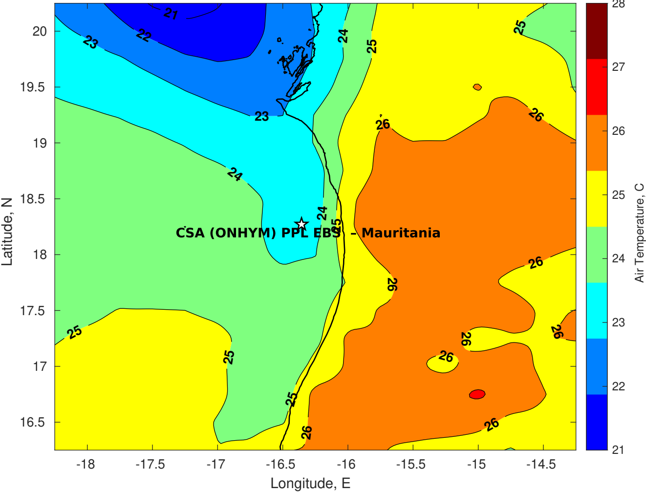
Air Temperature (C) for CSA (ONHYM) PPL EBS - Mauritania at 06-Dec-2025
