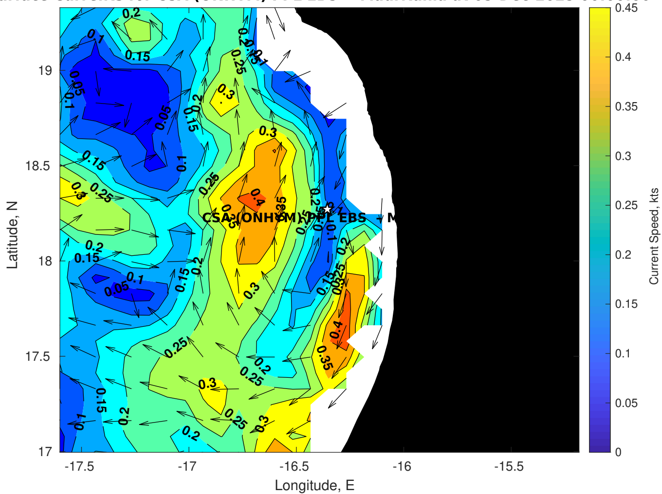
Surface Currents for CSA (ONHYM) PPL EBS - Mauritania at 05-Dec-2025 00:00:00
