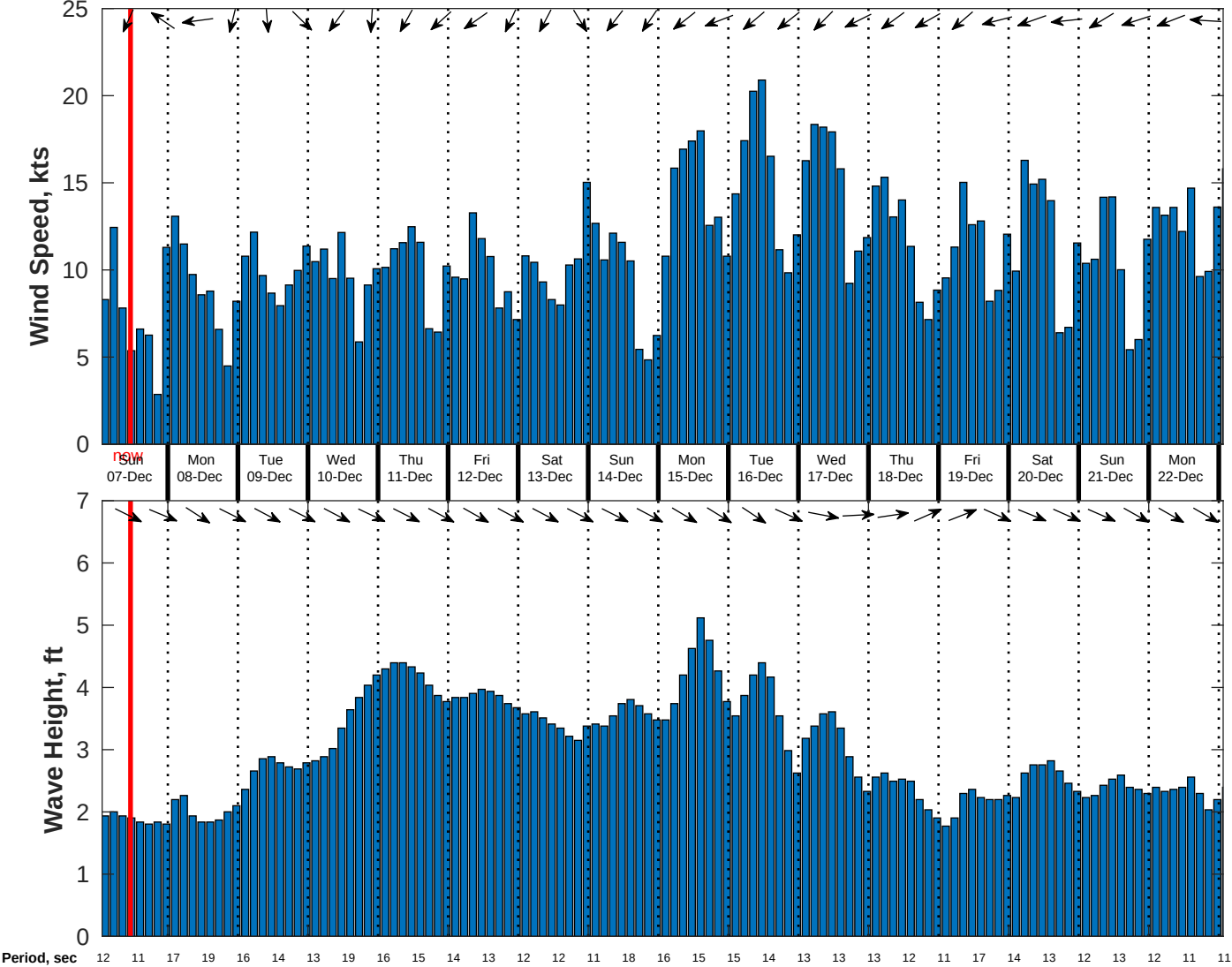
Wind & Wave Forecast for CSA (ONHYM) PPL EBS - Mauritania from 06-Dec-2025 01:00:00 to 22-Dec-2025 01:00:00
