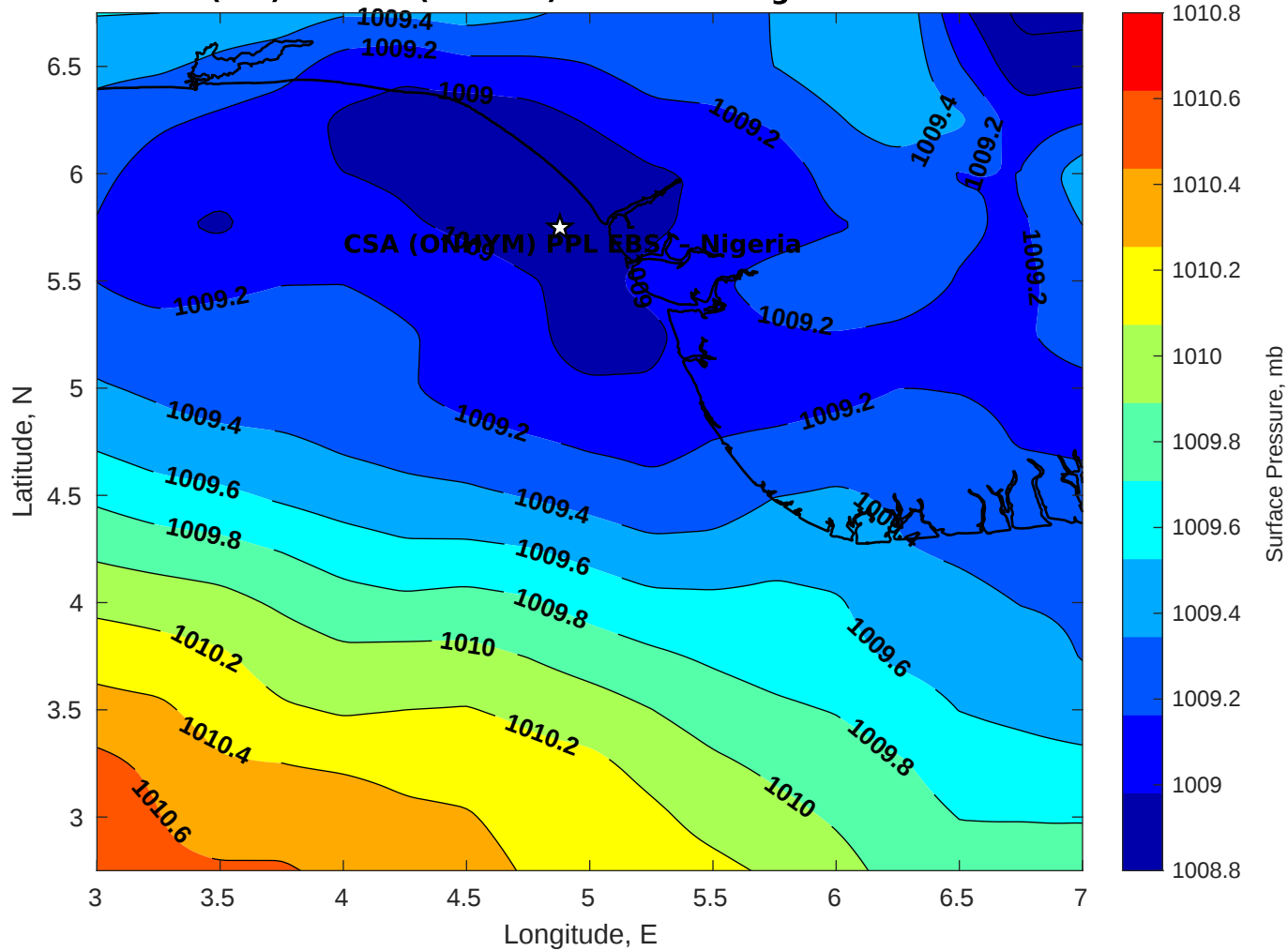
Surface Pressure (mb) for CSA (ONHYM) PPL EBS - Nigeria at 08-Dec-2025 00:00:00
