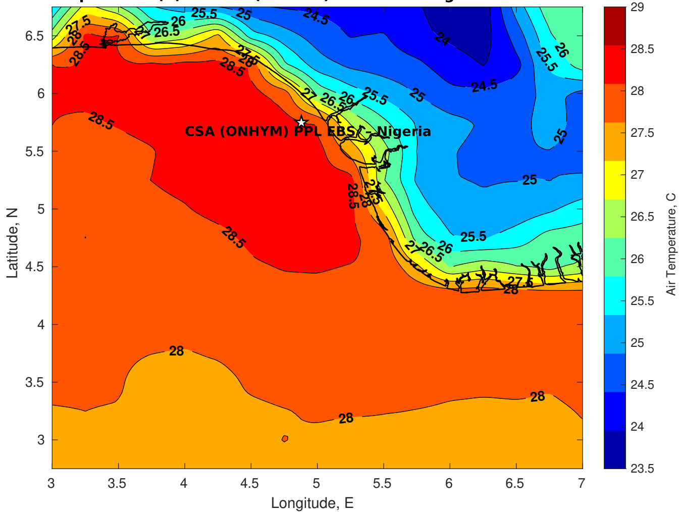
Air Temperature (C) for CSA (ONHYM) PPL EBS - Nigeria at 06-Dec-2025
