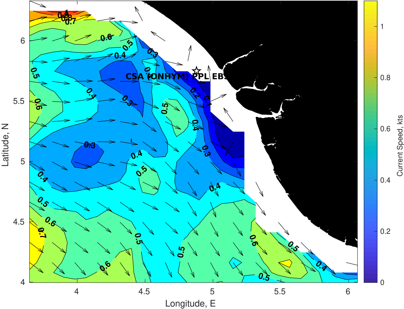
Surface Currents for CSA (ONHYM) PPL EBS - Nigeria at 05-Dec-2025 00:00:00
