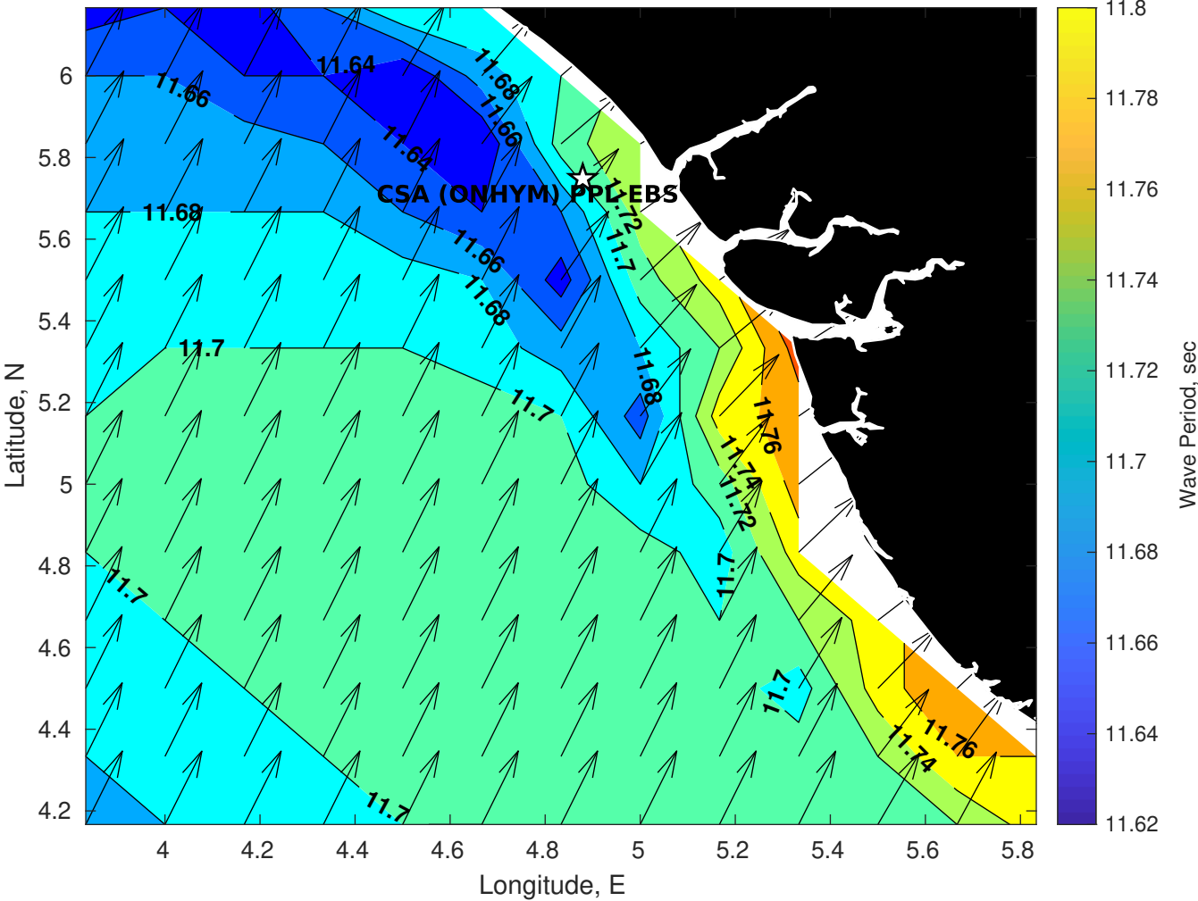
GFS Wave Period (sec) for CSA (ONHYM) PPL EBS - Nigeria at 06-Dec-2025 09:00:00
