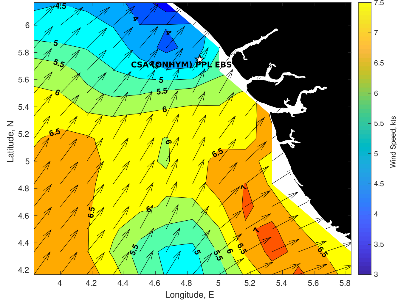
GFS Winds (kts) for CSA (ONHYM) PPL EBS - Nigeria at 06-Dec-2025 09:00:00
