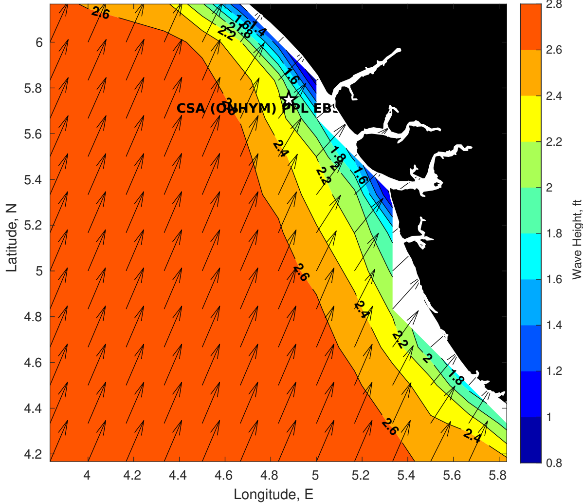
GFS Wave Height (ft) for CSA (ONHYM) PPL EBS - Nigeria at 06-Dec-2025 09:00:00
