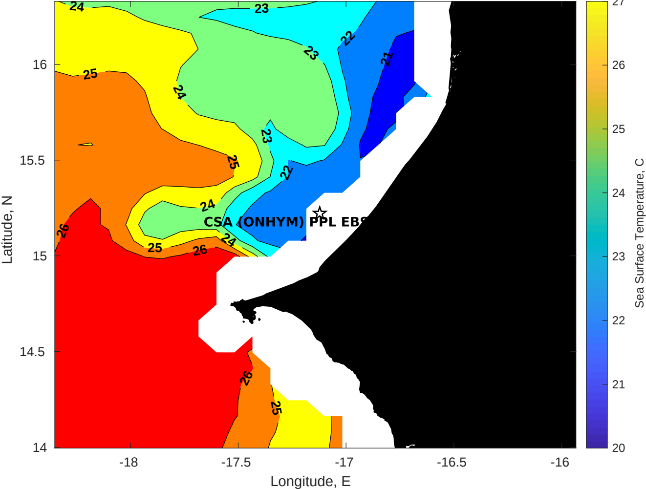
SST for CSA (ONHYM) PPL EBS - Senegal at 05-Dec-2025 00:00:00
