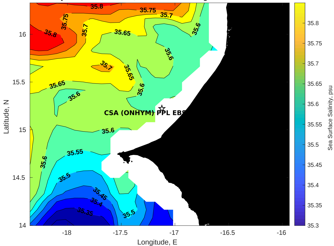
Surface Salinity for CSA (ONHYM) PPL EBS - Senegal at 05-Dec-2025 00:00:00
