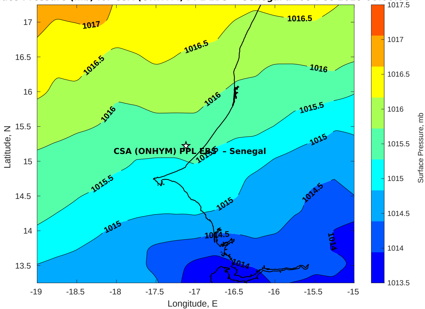
Surface Pressure (mb) for CSA (ONHYM) PPL EBS - Senegal at 08-Dec-2025 00:00:00
