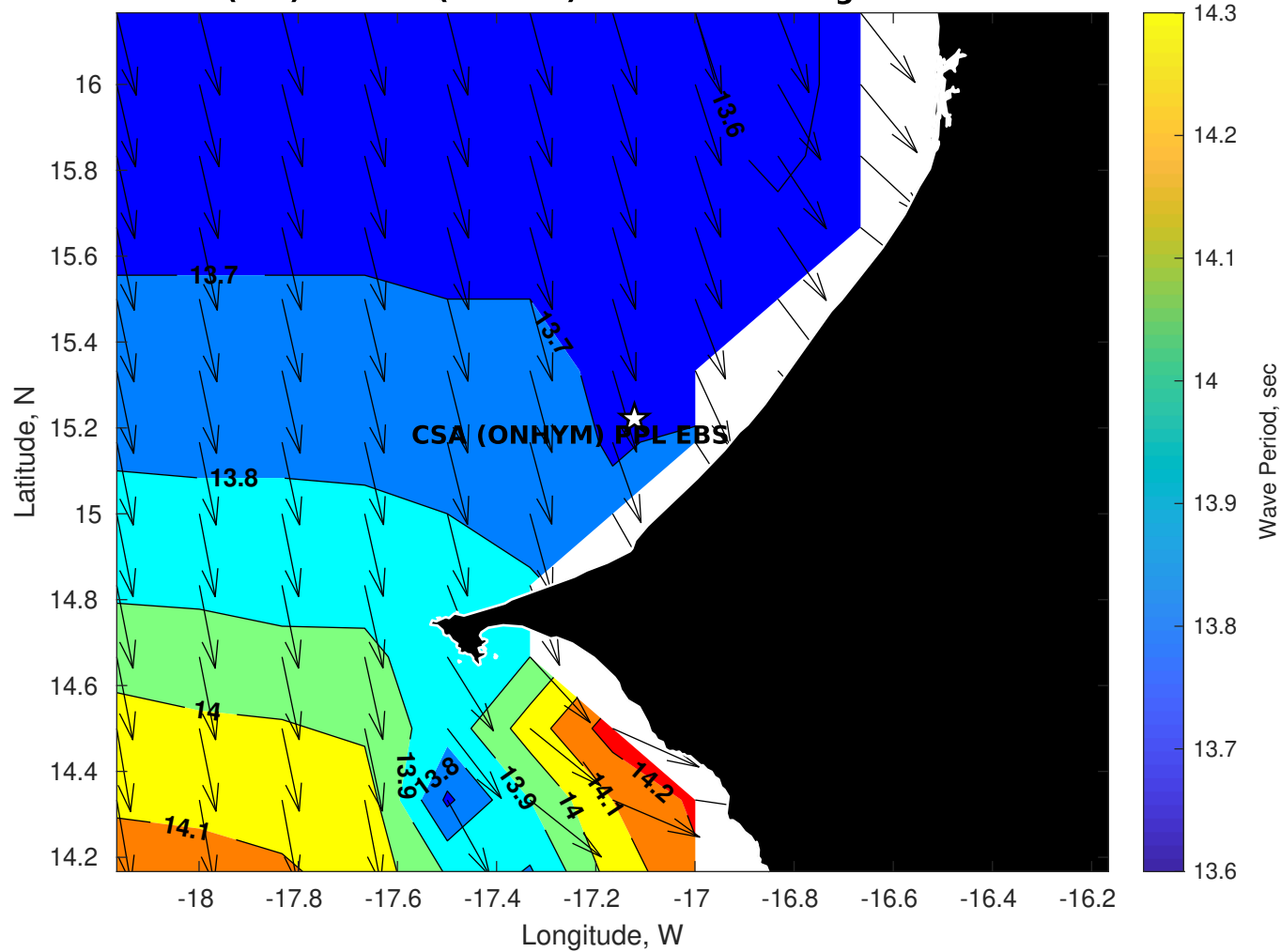
GFS Wave Period (sec) for CSA (ONHYM) PPL EBS - Senegal at 06-Dec-2025 09:00:00
