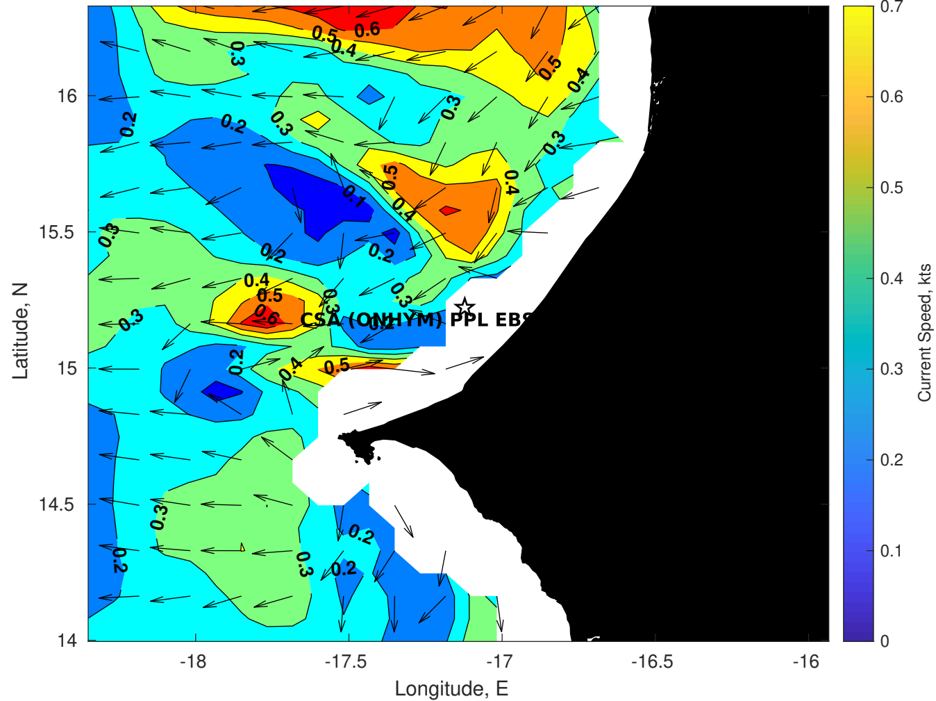
Surface Currents for CSA (ONHYM) PPL EBS - Senegal at 05-Dec-2025 00:00:00
