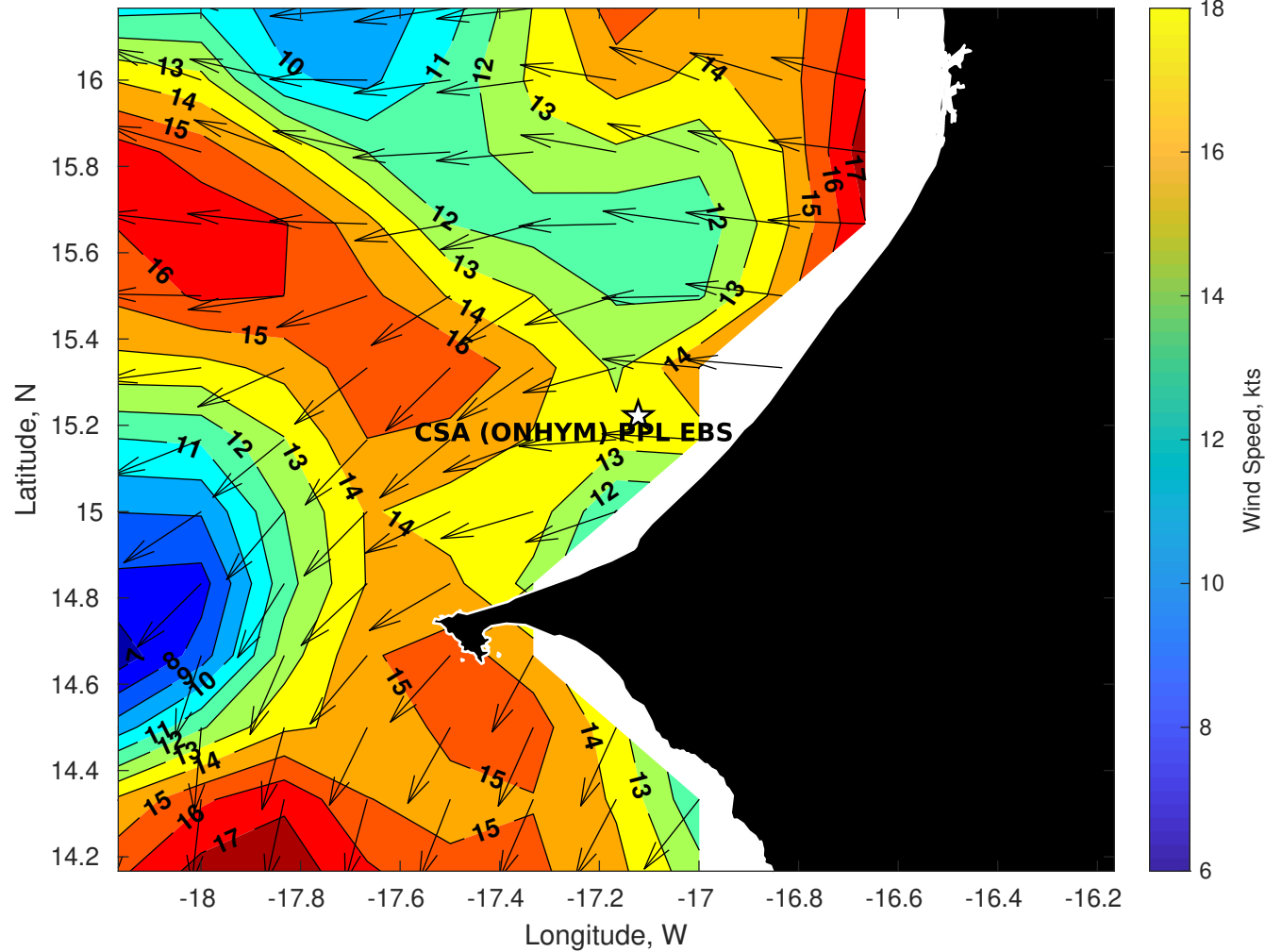
GFS Winds (kts) for CSA (ONHYM) PPL EBS - Senegal at 06-Dec-2025 09:00:00
