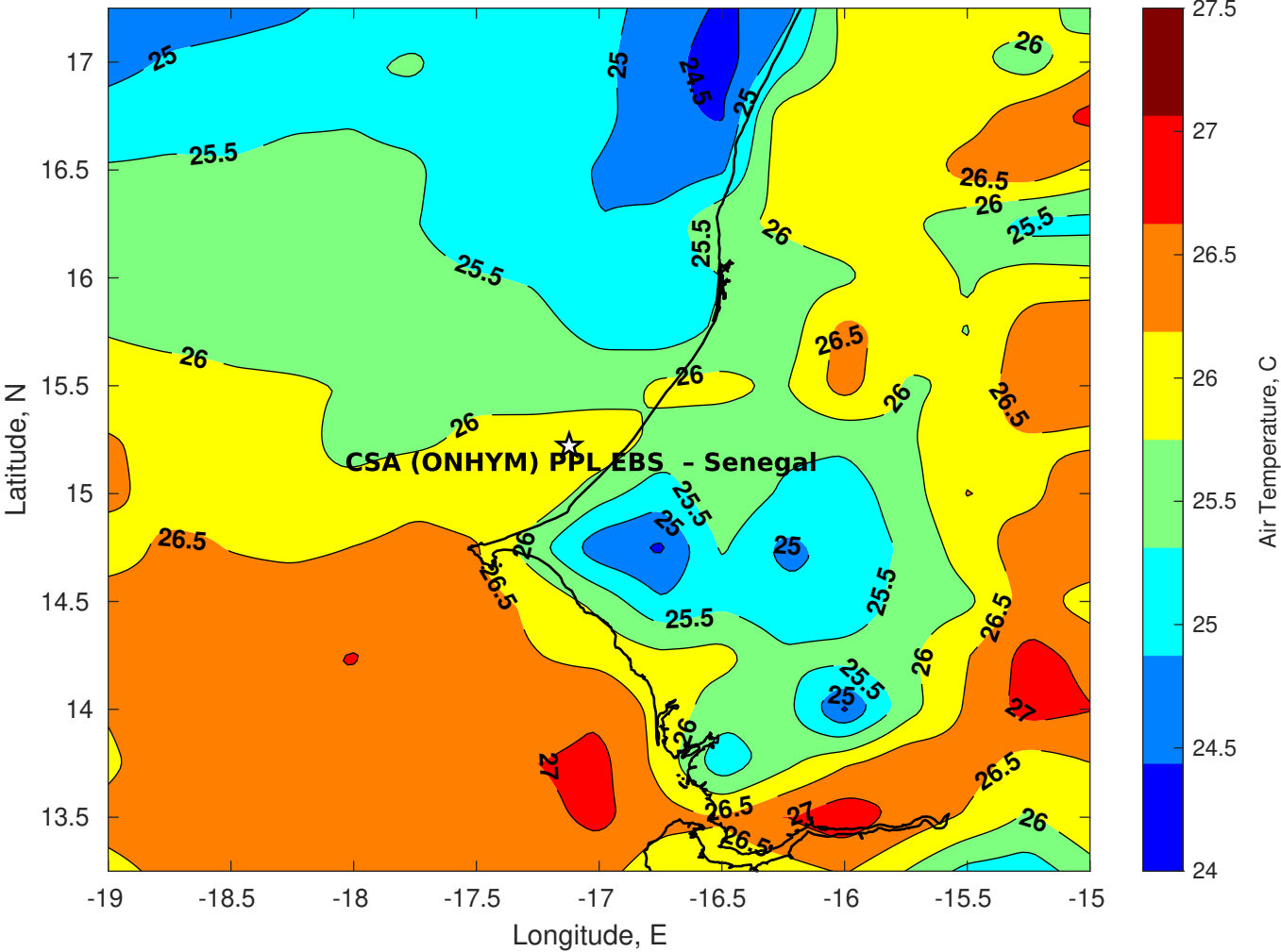
Air Temperature (C) for CSA (ONHYM) PPL EBS - Senegal at 06-Dec-2025
