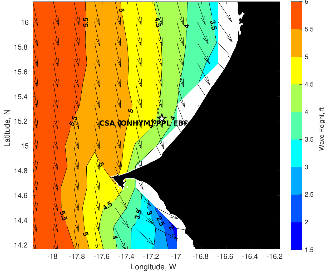
GFS Wave Height (ft) for CSA (ONHYM) PPL EBS - Senegal at 06-Dec-2025 09:00:00
