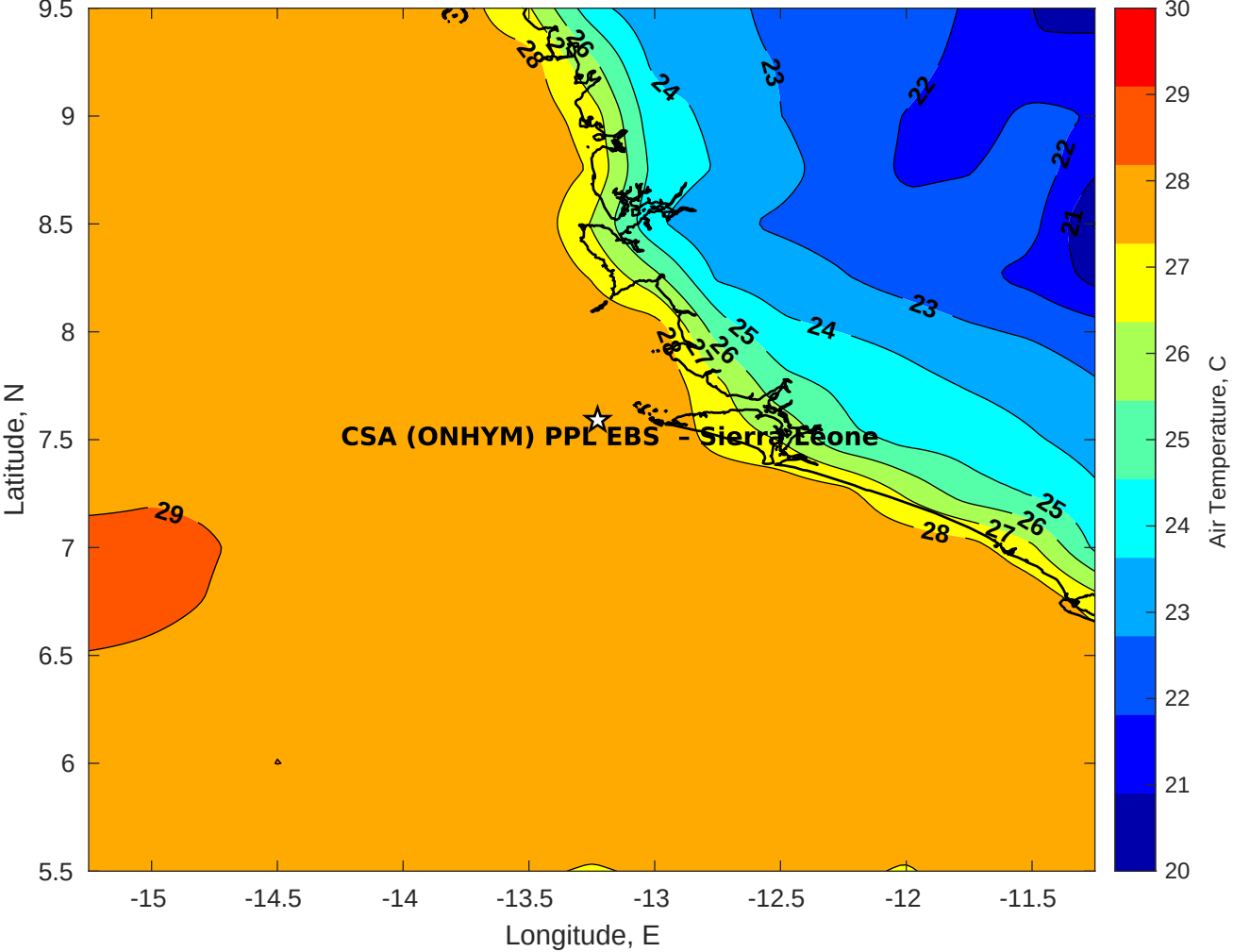
Air Temperature (C) for CSA (ONHYM) PPL EBS - Sierra Leone at 06-Dec-2025
