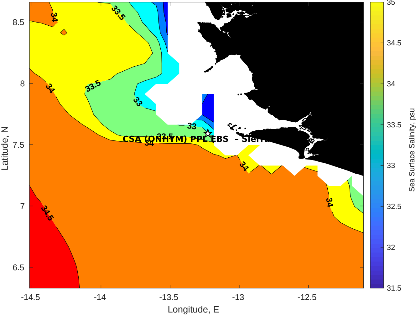
Surface Salinity for CSA (ONHYM) PPL EBS - Sierra Leone at 05-Dec-2025 00:00:00
