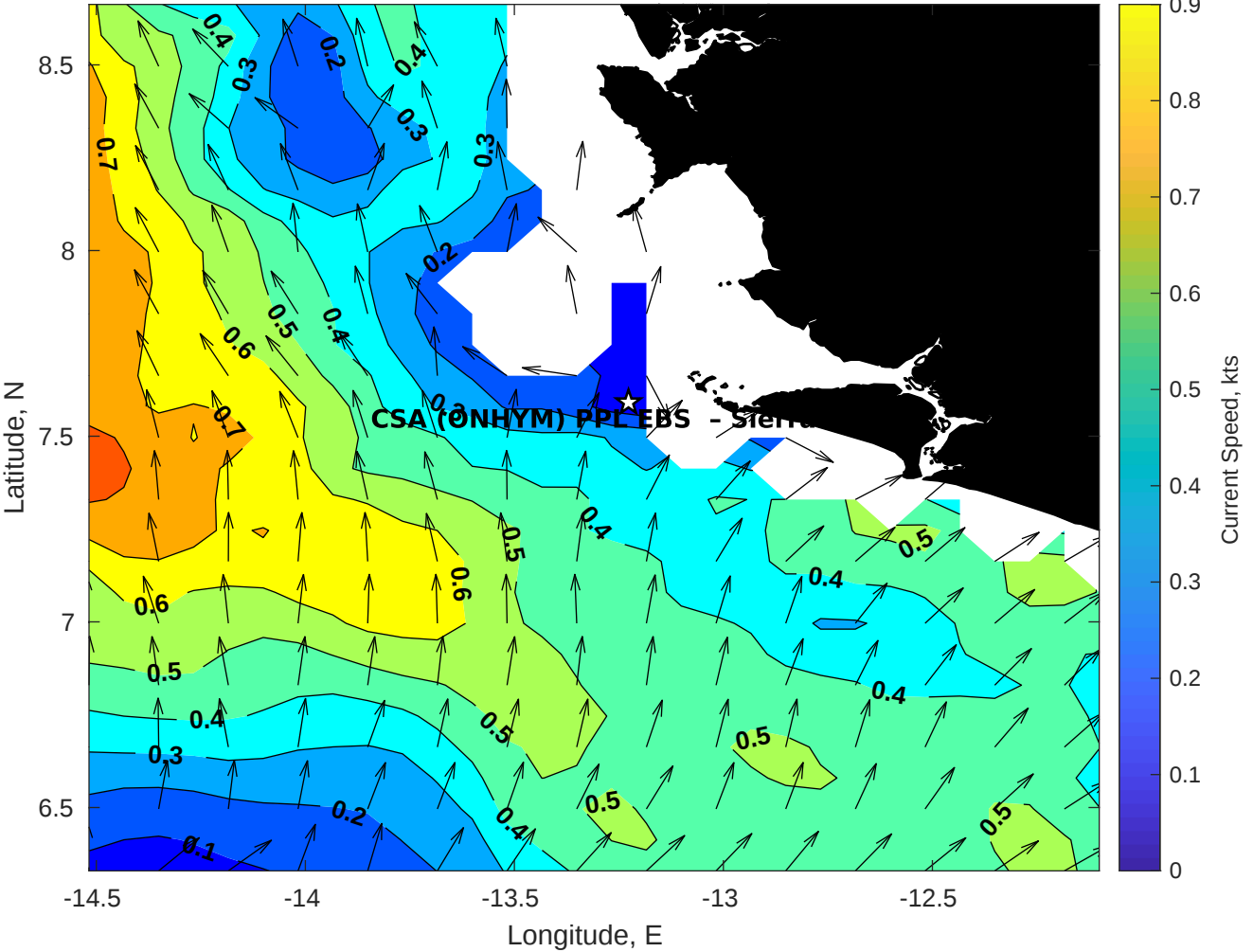
Surface Currents for CSA (ONHYM) PPL EBS - Sierra Leone at 05-Dec-2025 00:00:00
