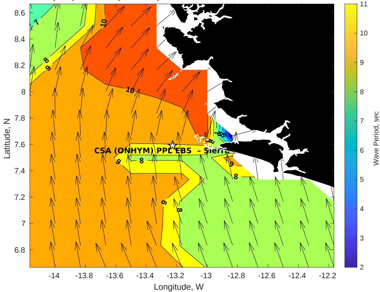
GFS Wave Period (sec) for CSA (ONHYM) PPL EBS - Sierra Leone at 06-Dec-2025 09:00:00
