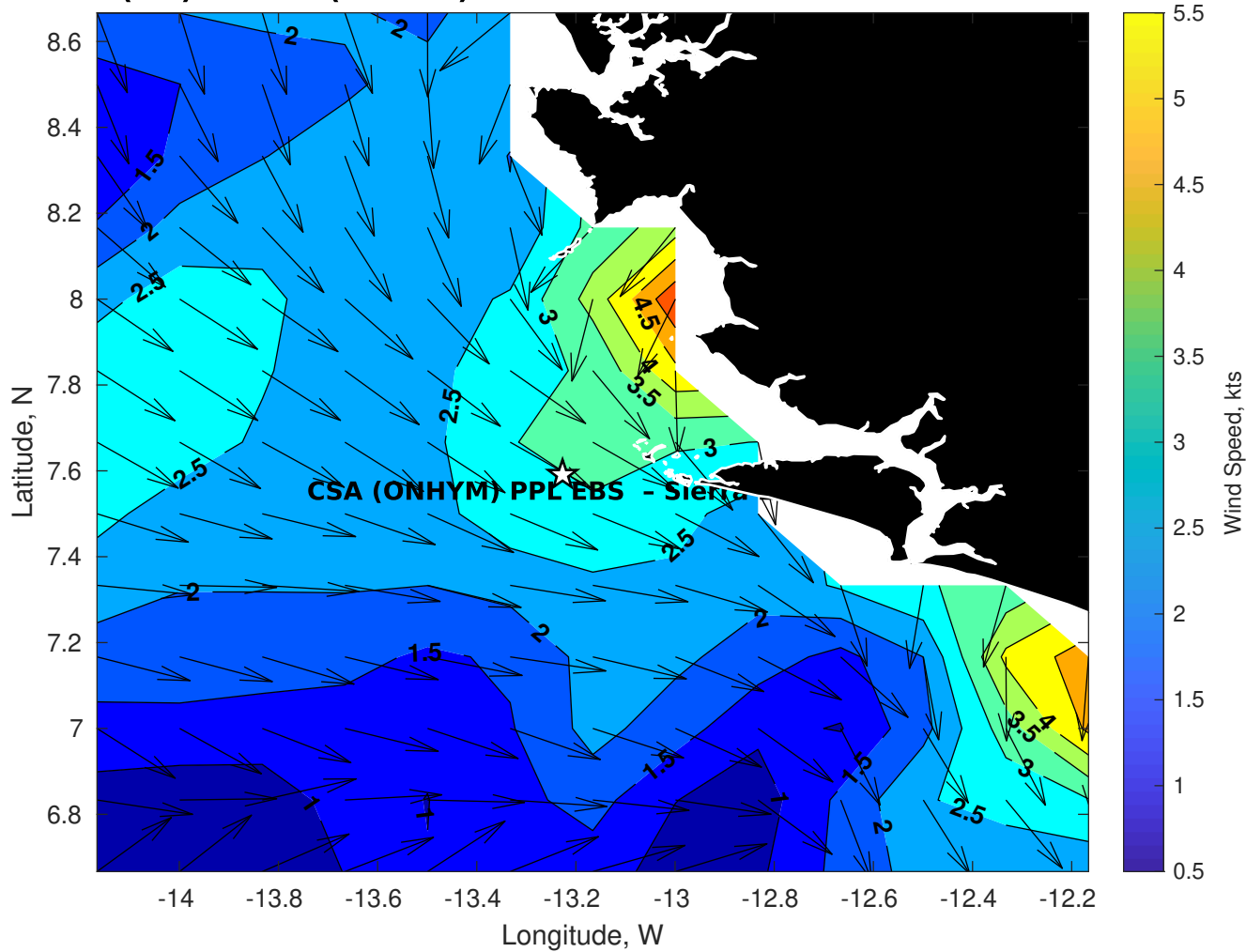
GFS Winds (kts) for CSA (ONHYM) PPL EBS - Sierra Leone at 06-Dec-2025 09:00:00
