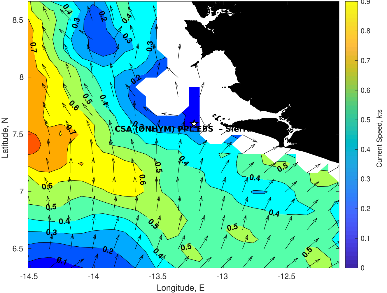
Surface Currents for CSA (ONHYM) PPL EBS - Sierra Leone at 05-Dec-2025 00:00:00
