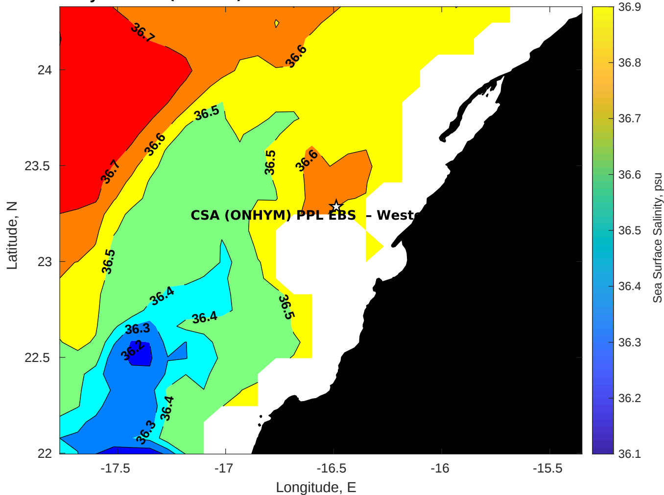
Surface Salinity for CSA (ONHYM) PPL EBS - Western Sahara at 05-Dec-2025 00:00:00
