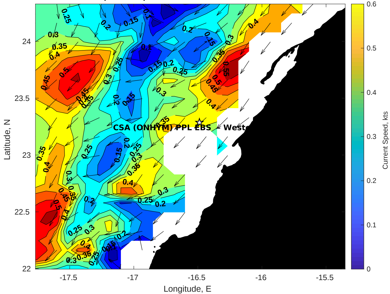
Surface Currents for CSA (ONHYM) PPL EBS - Western Sahara at 05-Dec-2025 00:00:00
