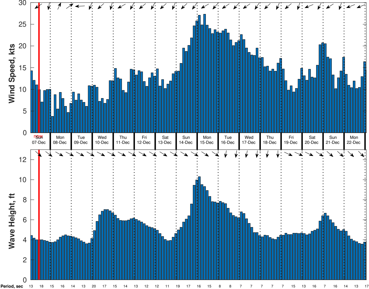
Wind & Wave Forecast for CSA (ONHYM) PPL EBS - Western Sahara from 06-Dec-2025 01:00:00 to 22-Dec-2025 01:00:00
