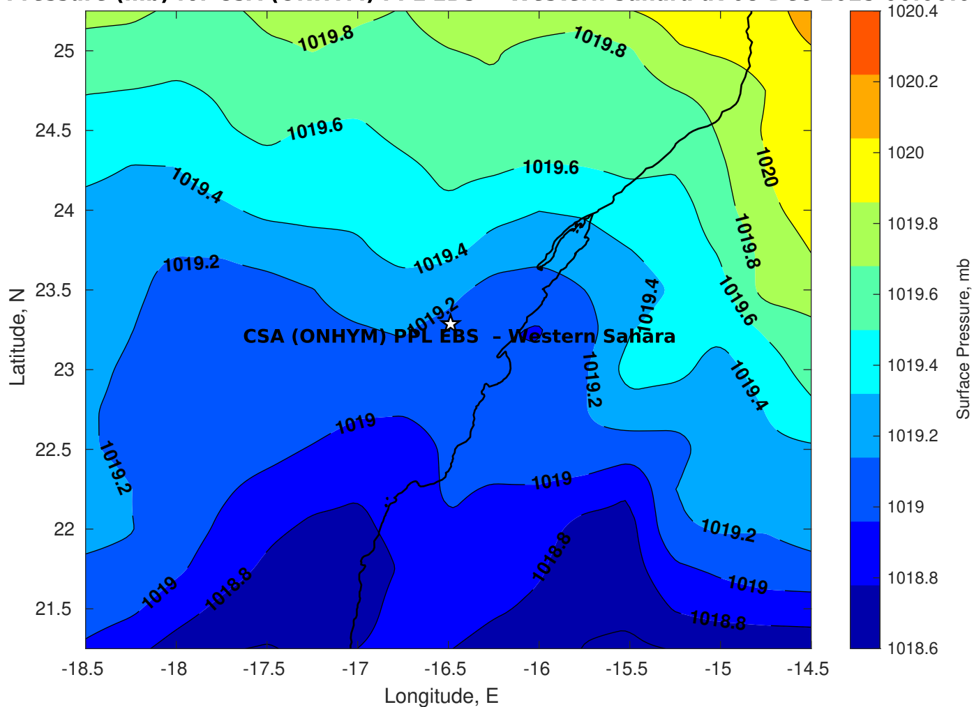
Surface Pressure (mb) for CSA (ONHYM) PPL EBS - Western Sahara at 08-Dec-2025 00:00:00
