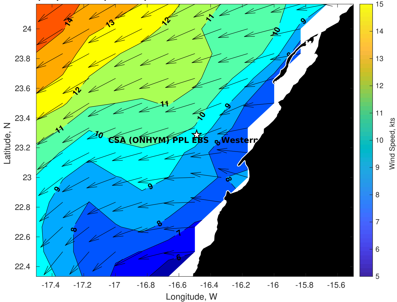
GFS Winds (kts) for CSA (ONHYM) PPL EBS - Western Sahara at 06-Dec-2025 09:00:00
