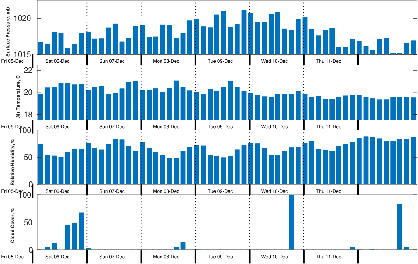
Met Forecast for CSA (ONHYM) PPL EBS - Western Sahara from 06-Dec-2025 00:00:00 to 13-Dec-2025 00:00:00
