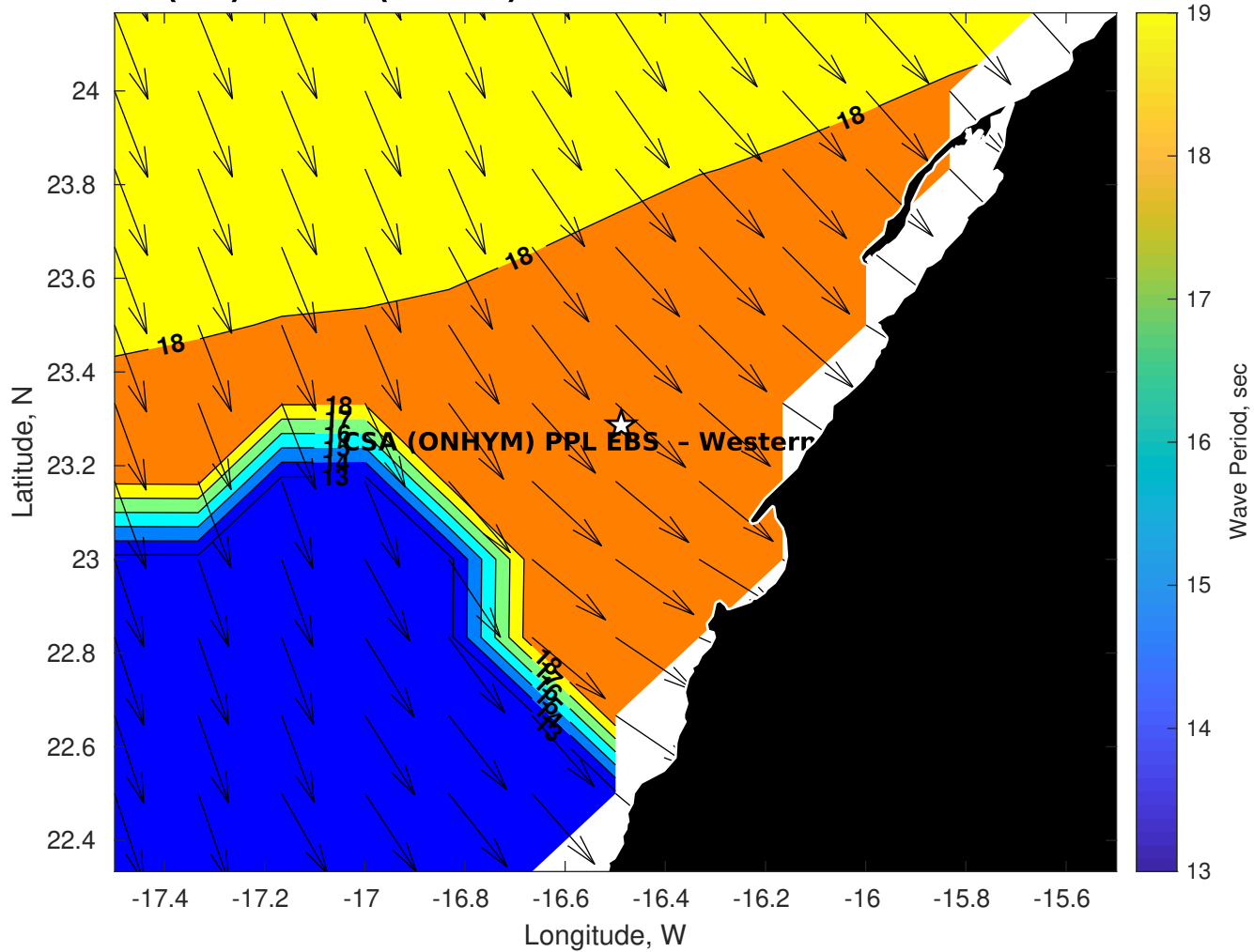
GFS Wave Period (sec) for CSA (ONHYM) PPL EBS - Western Sahara at 06-Dec-2025 09:00:00
