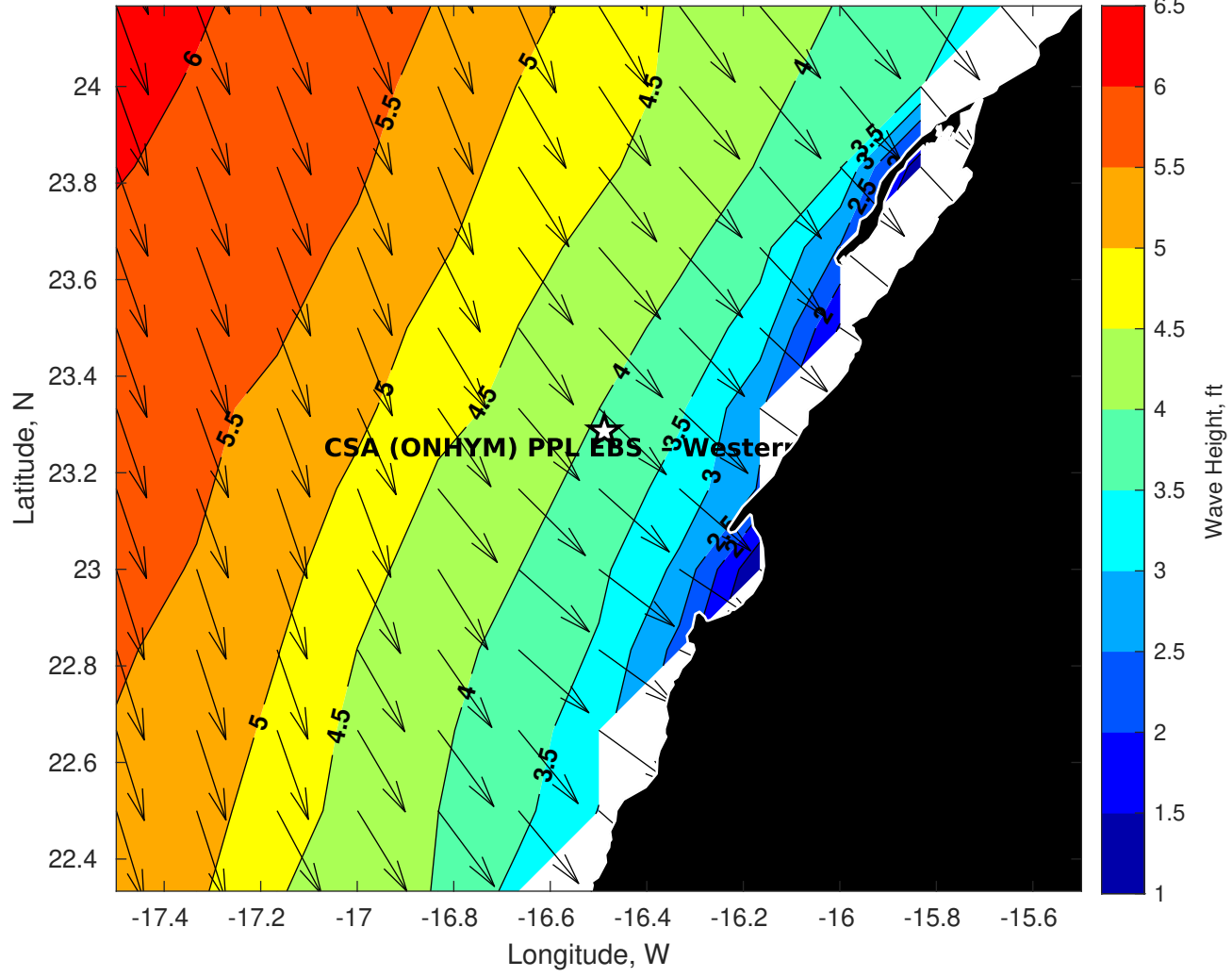
GFS Wave Height (ft) for CSA (ONHYM) PPL EBS - Western Sahara at 06-Dec-2025 09:00:00
