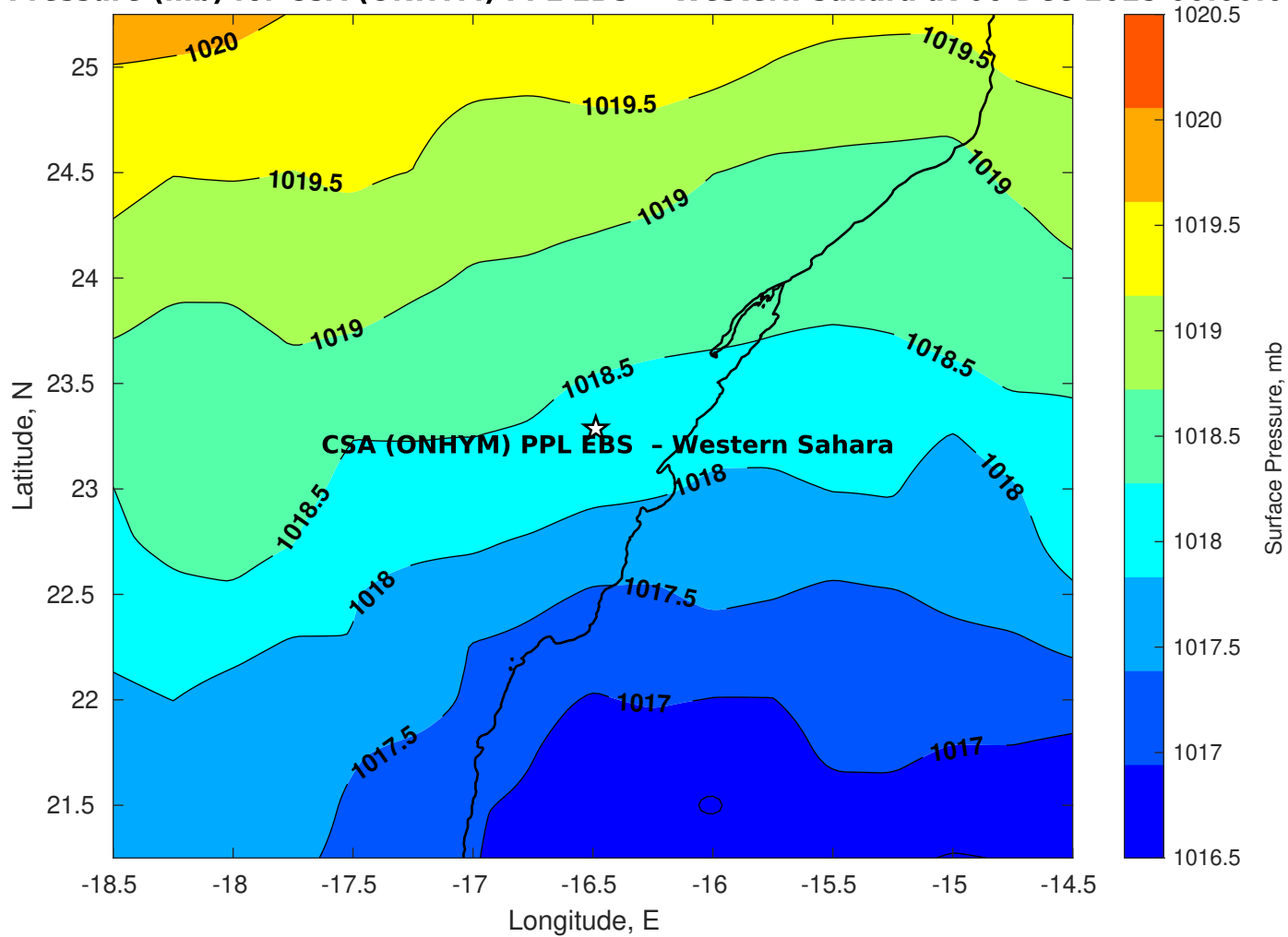
Surface Pressure (mb) for CSA (ONHYM) PPL EBS - Western Sahara at 06-Dec-2025 00:00:00
