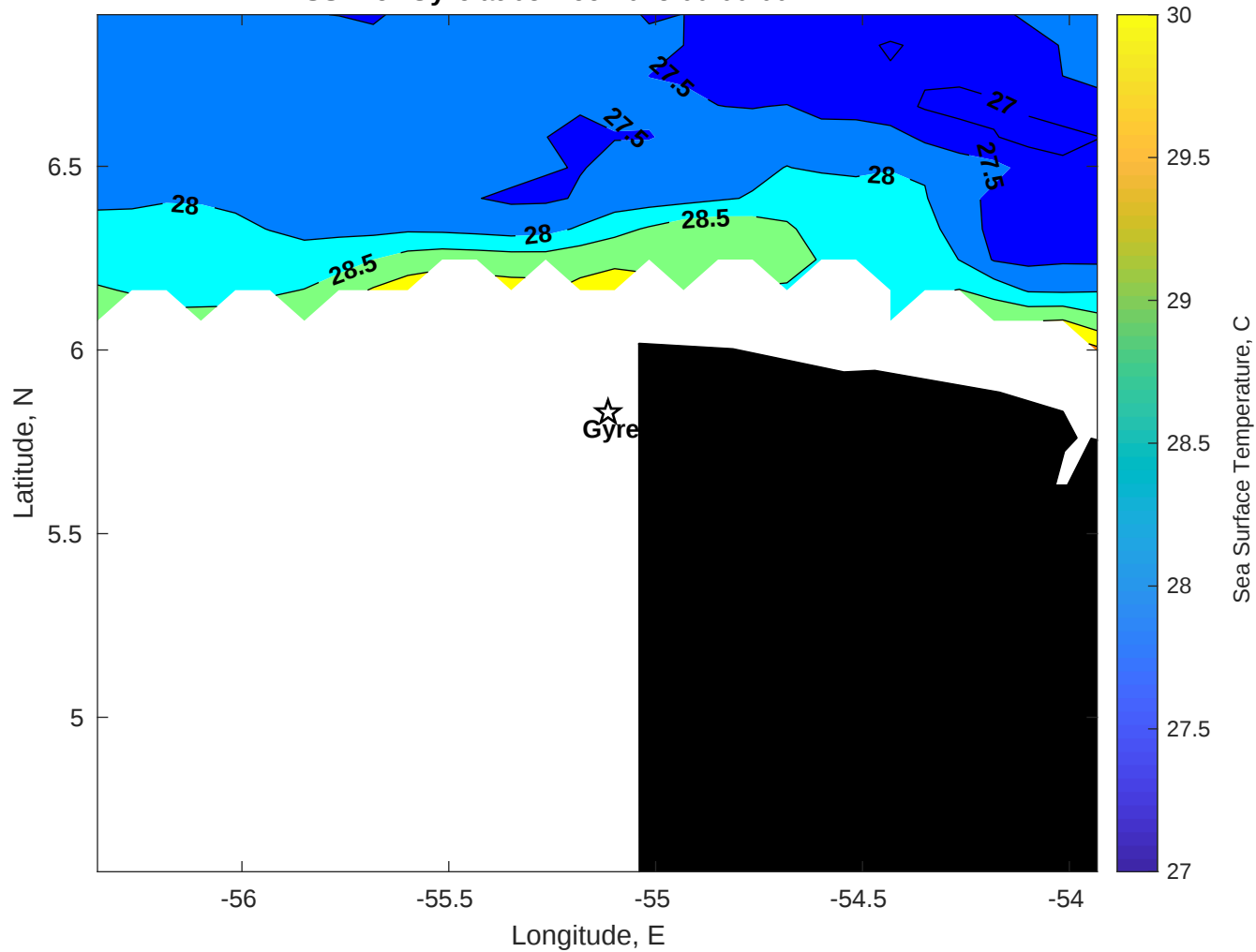
SST for Gyre at 05-Dec-2025 00:00:00
