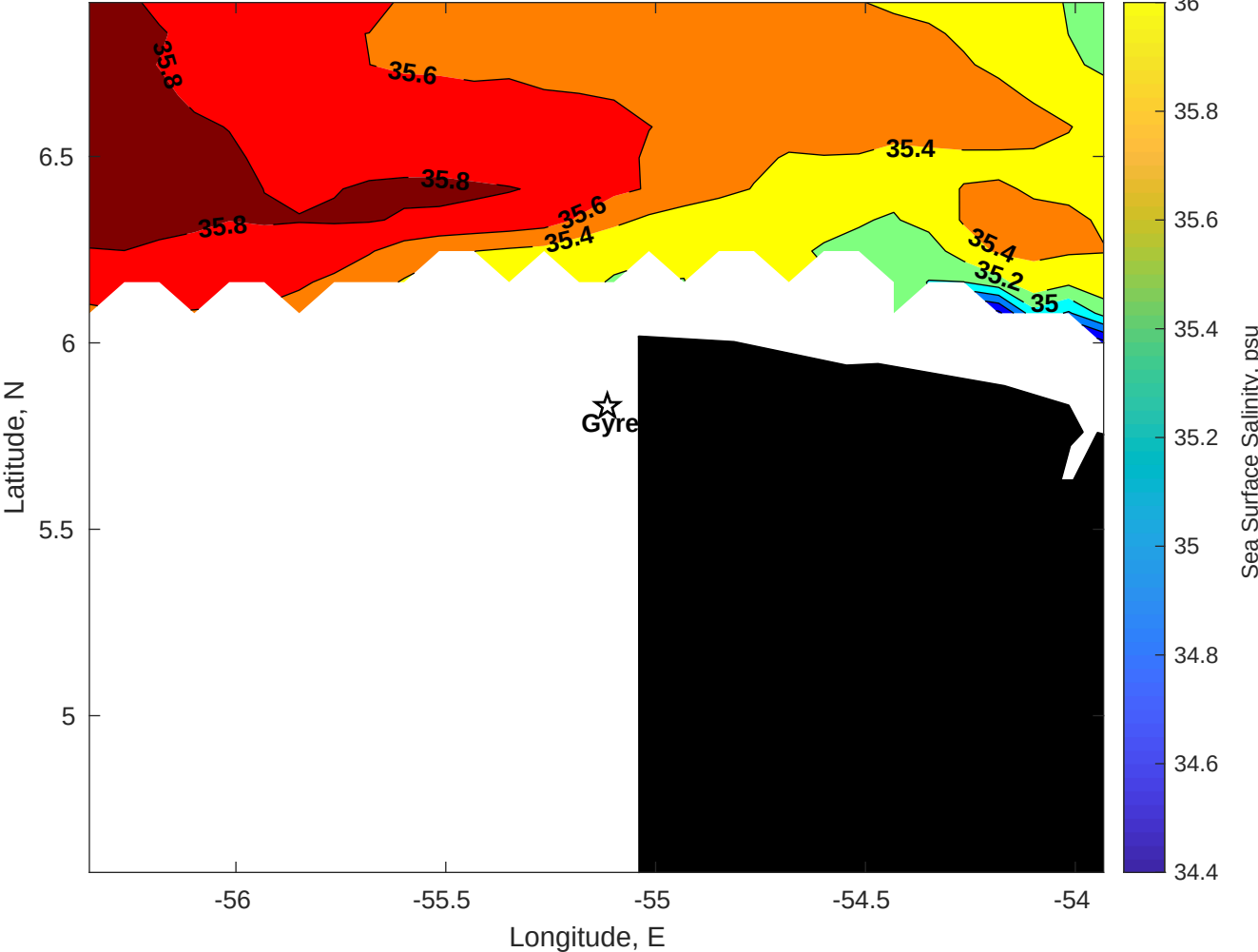
Surface Salinity for Gyre at 05-Dec-2025 00:00:00
