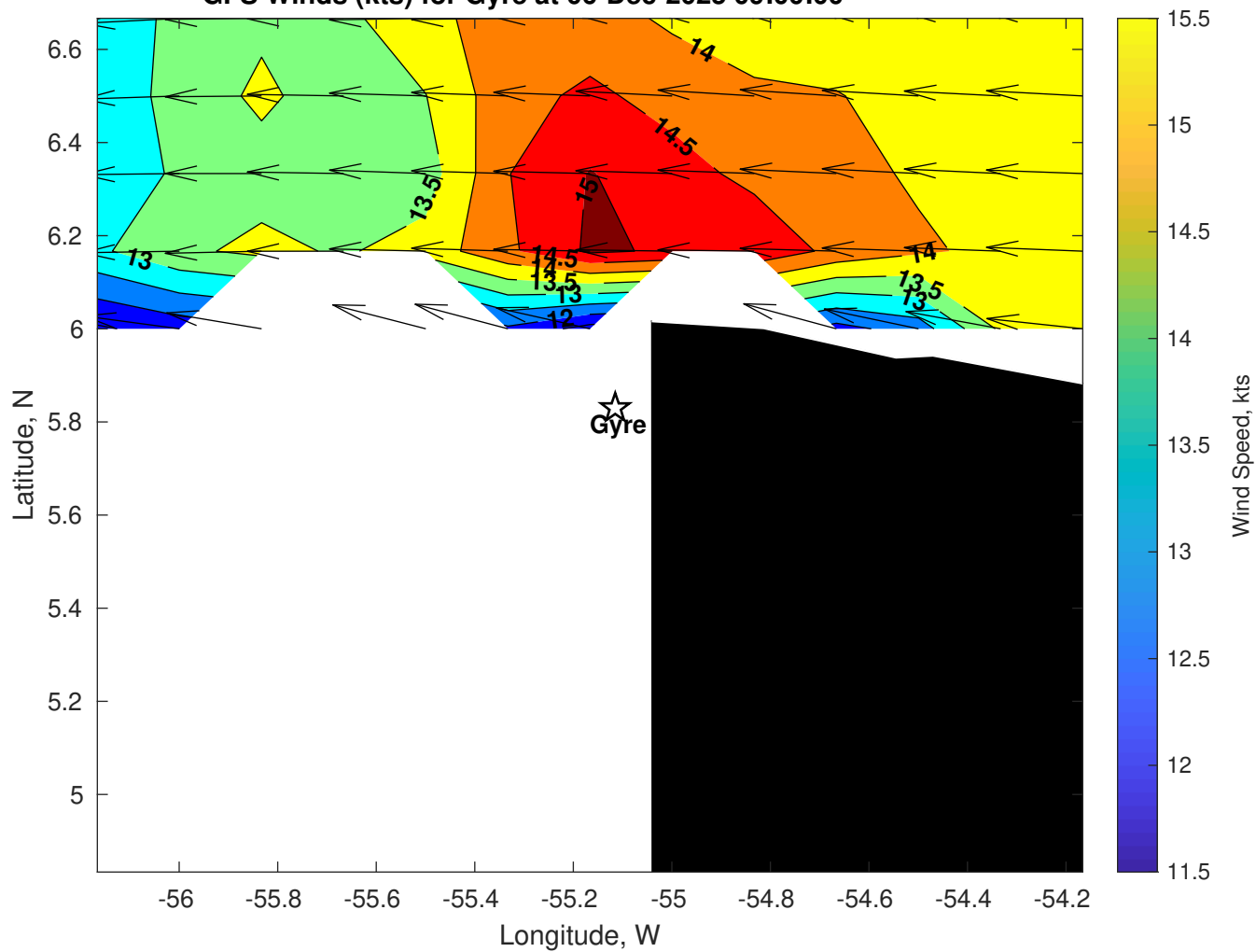
GFS Winds (kts) for Gyre at 06-Dec-2025 09:00:00
