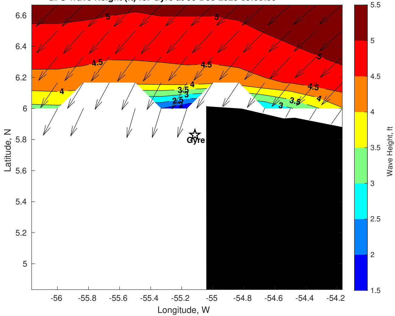
GFS Wave Height (ft) for Gyre at 06-Dec-2025 09:00:00
