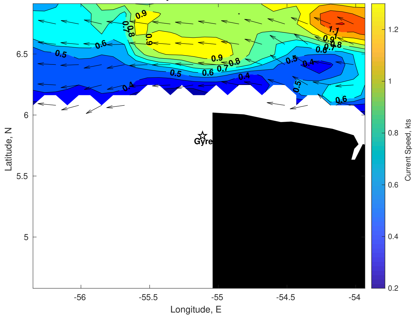
Surface Currents for Gyre at 05-Dec-2025 00:00:00
