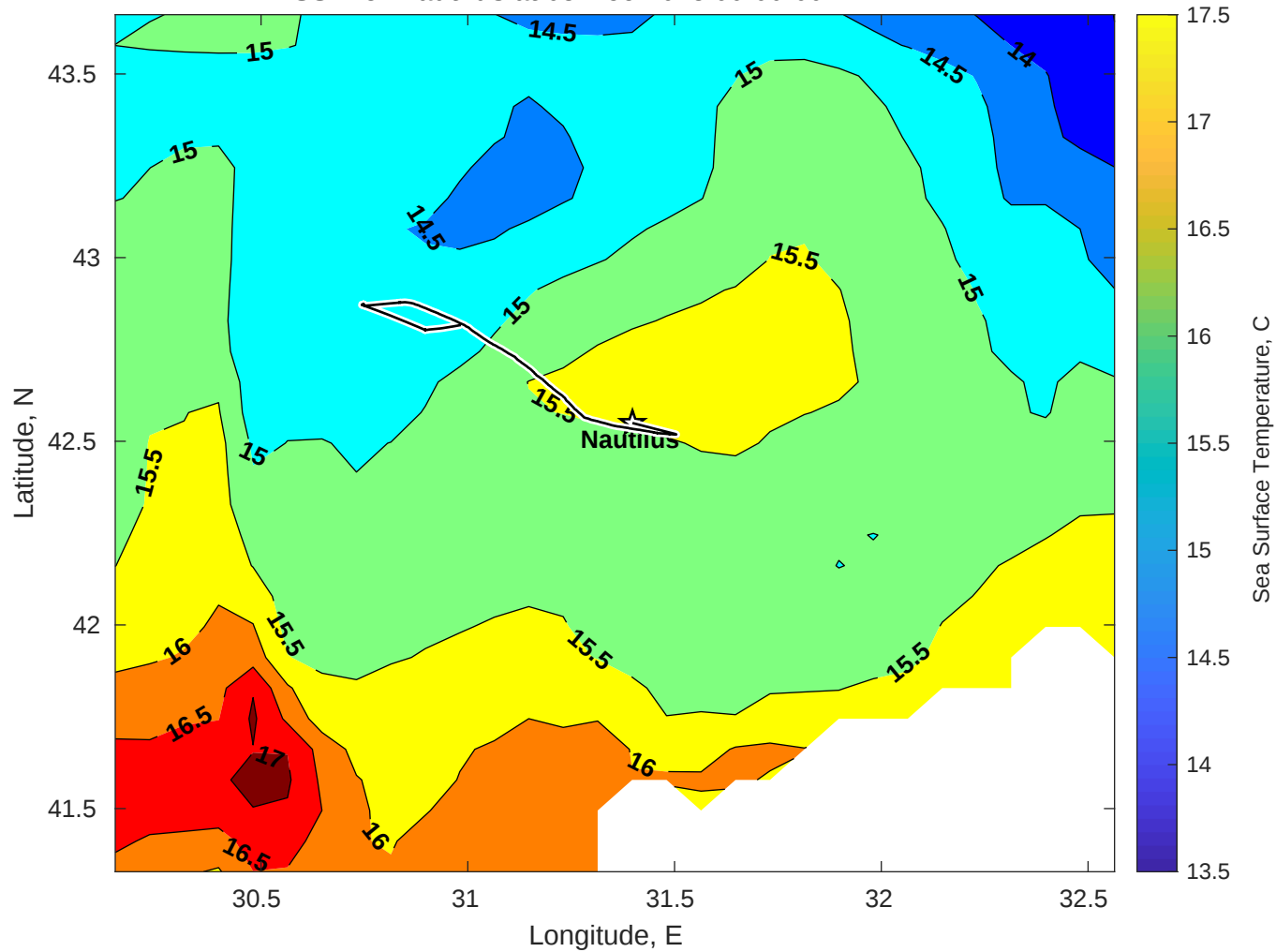
SST for Nautilus at 05-Dec-2025 00:00:00
