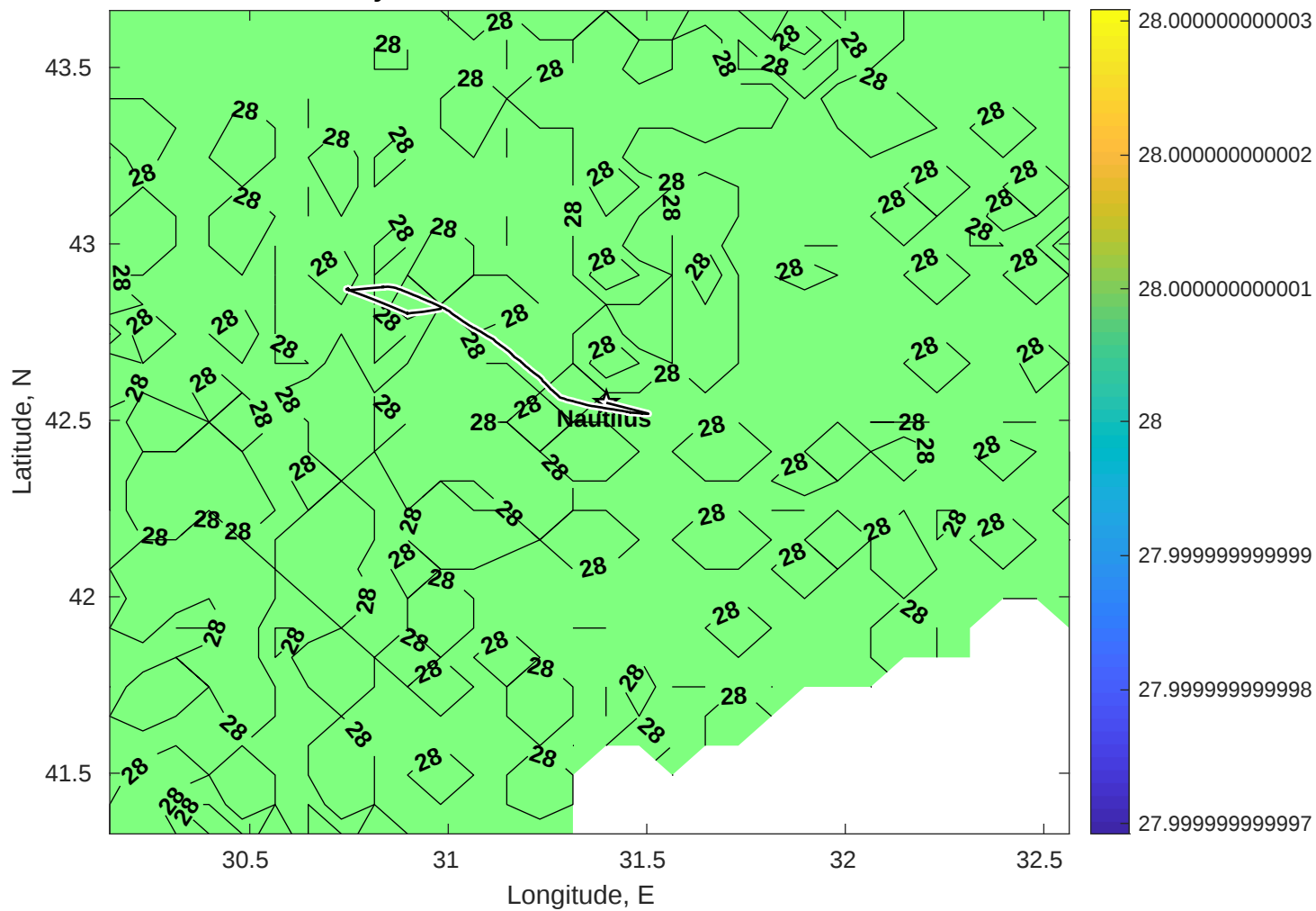
Surface Salinity for Nautilus at 05-Dec-2025 00:00:00
