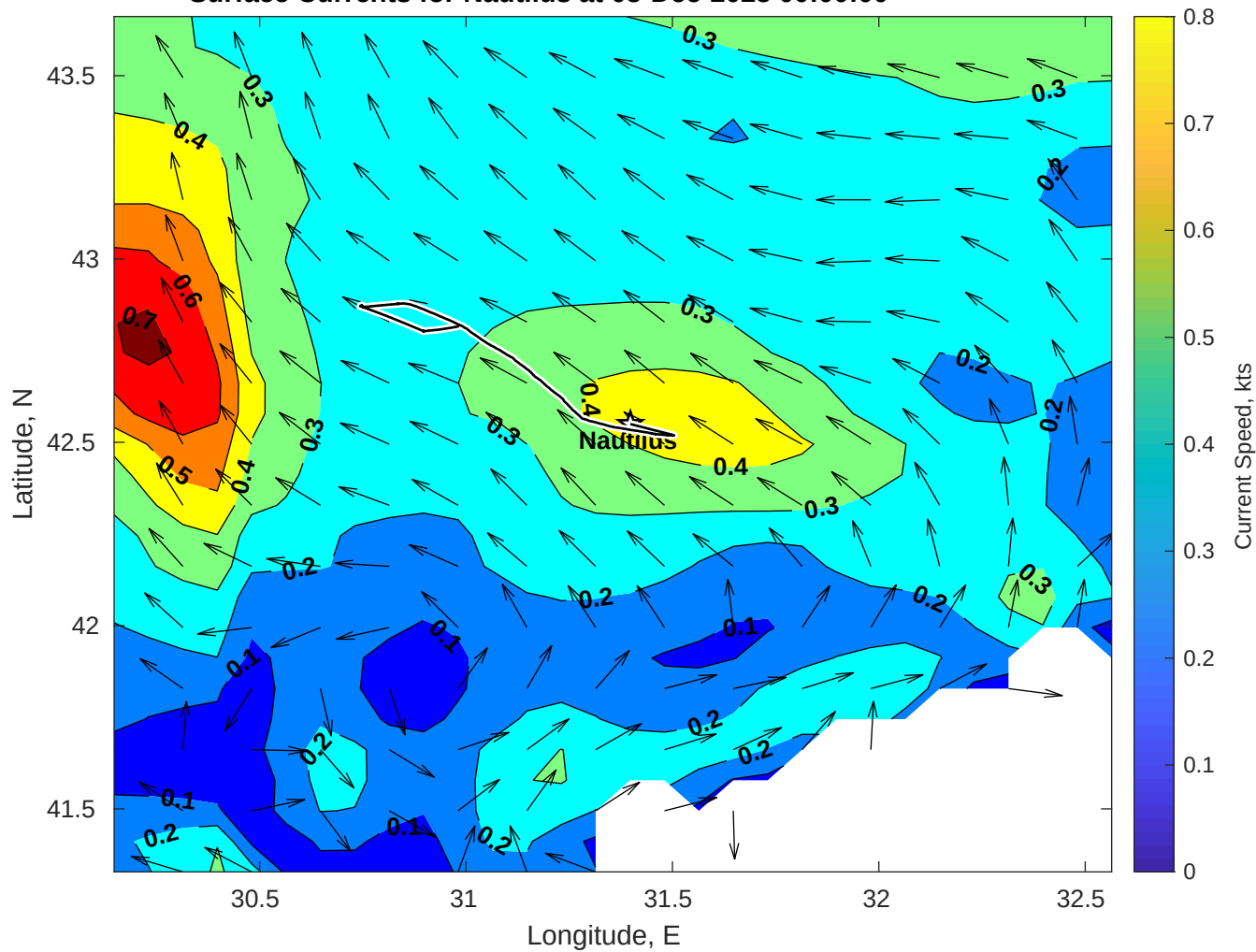
Surface Currents for Nautilus at 05-Dec-2025 00:00:00
