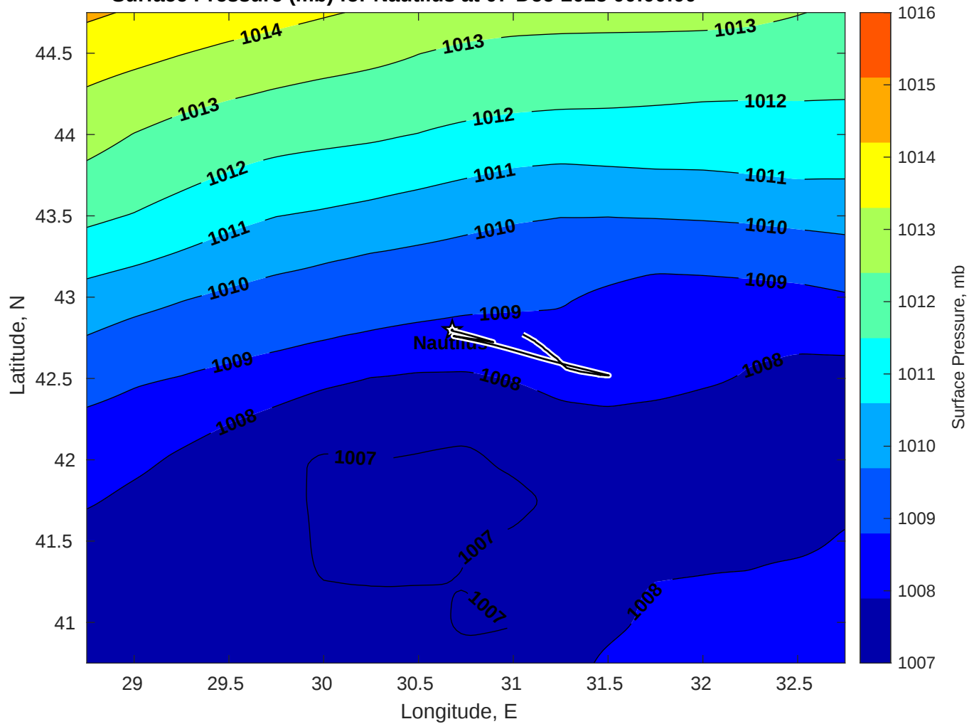
Surface Pressure (mb) for Nautilus at 07-Dec-2025 00:00:00
